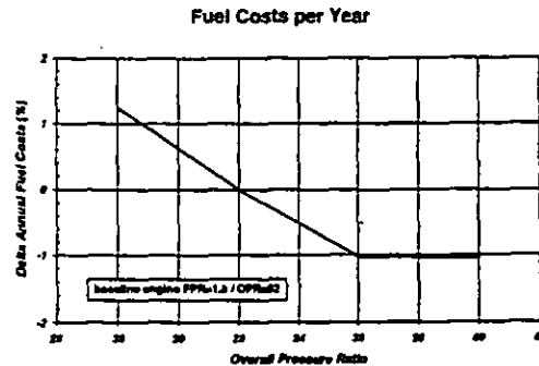
Figure 9. Annual Fuel Costs
