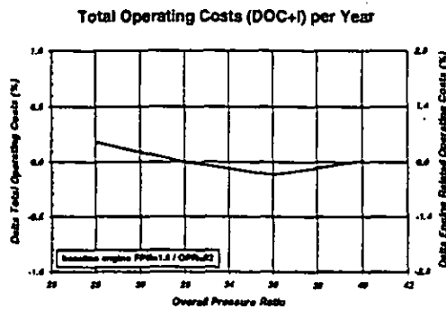
Figure 10. Annual Operating Costs
