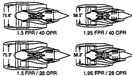
Figure 5. Effect of Engine Cycle on Size at Constant Takeoff and Top of Climb Thrust
