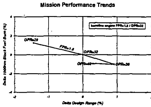
Figure 6. Mission Performance Trends
