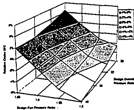
Figure 3. Effect of Fan Pressure Ratio and Overall Pressure Ratio on Cruise SFC
