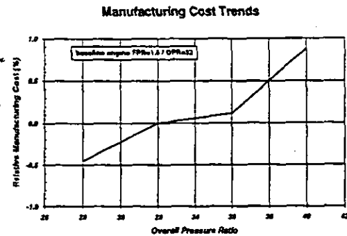
Figure 8. Effect of Overall Pressure Ratio on Manufacturing Cost
