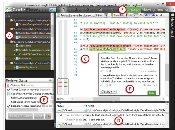
Fig. 1: Example of Code Review using CodeFlow
