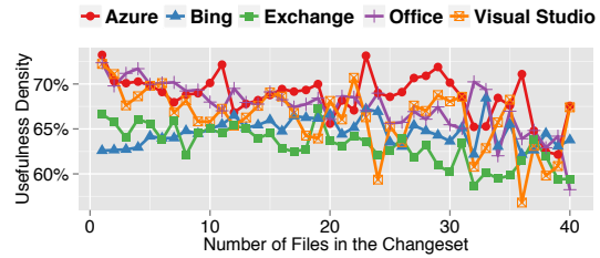
Fig. 8: Usefulness density vs. Number of files
