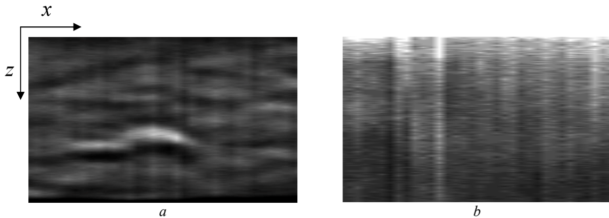
Figure 3 – Laser ultrasonic structural images of Karelian marble sample ( x=30 mm, y=26 mm, z=28 mm): a – before heating; b – after heating to 700°C.
