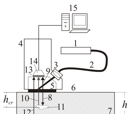
Figure 1 – The scheme of the laser optoacoustic transducer: 1 - the pulse solid laser, 2 - fibre-optical cable, 3 - optical system, 4 - the case of the laser optoacoustic transducer, 5 - transparent prism, 6 - optoacoustic generator, 7 - researched sample, 8 - probing pulse, 9 - reference pulse, 10 - pulse reflected from the defect, 11 - defect of structure of the sample, 12 - pulse reflected from the sample backside, 13 – damper piezo-receiver, 14 - preamplifier, 15 - computer system of data processing.
