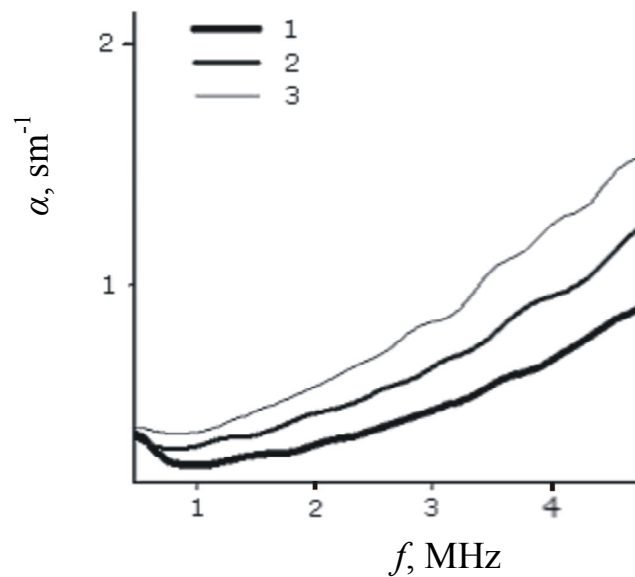
Figure 6 – Frequency dependences of ultrasonic attenuation factor in ferruginous quartzite sample: 1 - initial condition, 2 - after the first electromagnetic pulse influence (power P_1 ), 3- after the second electromagnetic pulse influence (power 4P_1 ).
