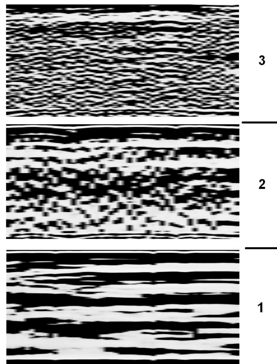
Figure 4 – Laser ultrasonic structural images of ferruginous quartzite sample: 1 - initial condition, 2 - after the first electromagnetic pulse influence (power P_1 ), 3- after the second electromagnetic pulse influence (power 4P_1 ).
