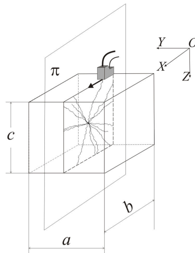
Figure 2 – The laser ultrasonic scanning scheme of the rock sample.
