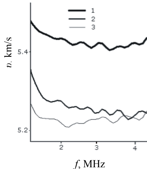
Figure 5 – Frequency dependences of longitudinal wave velocity in ferruginous quartzite sample: 1 - initial condition, 2 - after the first electromagnetic pulse influence (power P_1 ), 3 - after the second electromagnetic pulse influence (power 4P_1 ).
