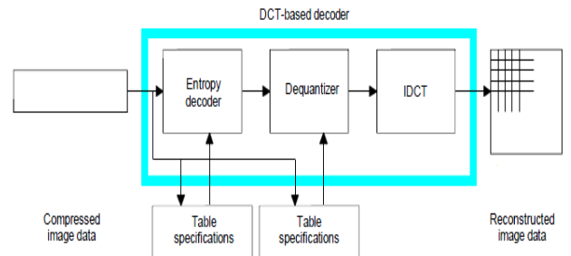
Figure 5: JPEG Decoder [5].
