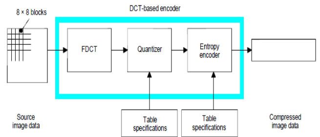
Figure 4: JPEG Encoder [5].
