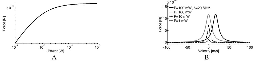
FIGURE 3. Photon scattering force vs. A) incident laser power and B) vs. atom velocity
