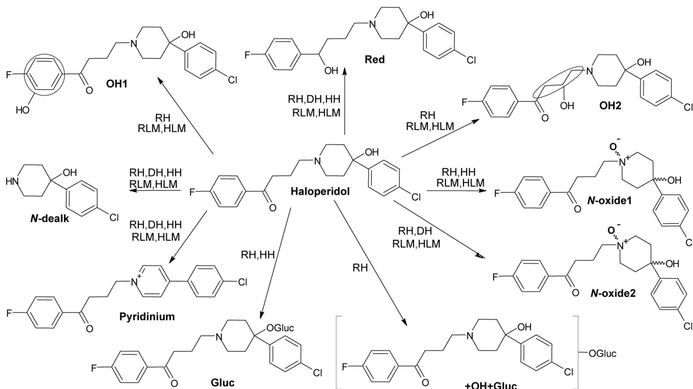
FIG. 2. Proposed overall metabolism of haloperidol in HLMs, RLMs, and hepatocytes (HH, human; DH, dog; RH, rat).
