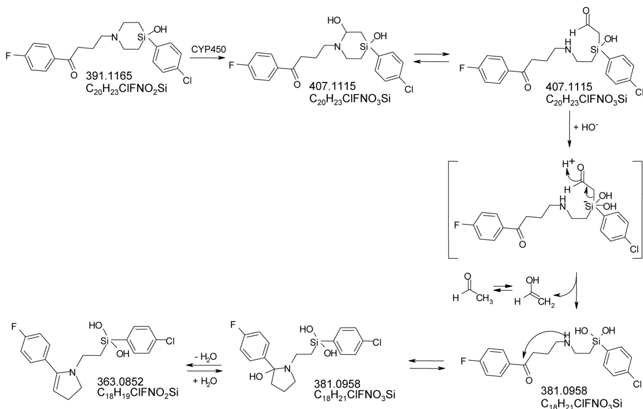
Fig. 9. Proposed mechanism for the metabolic ring opening of sila-haloperidol.
