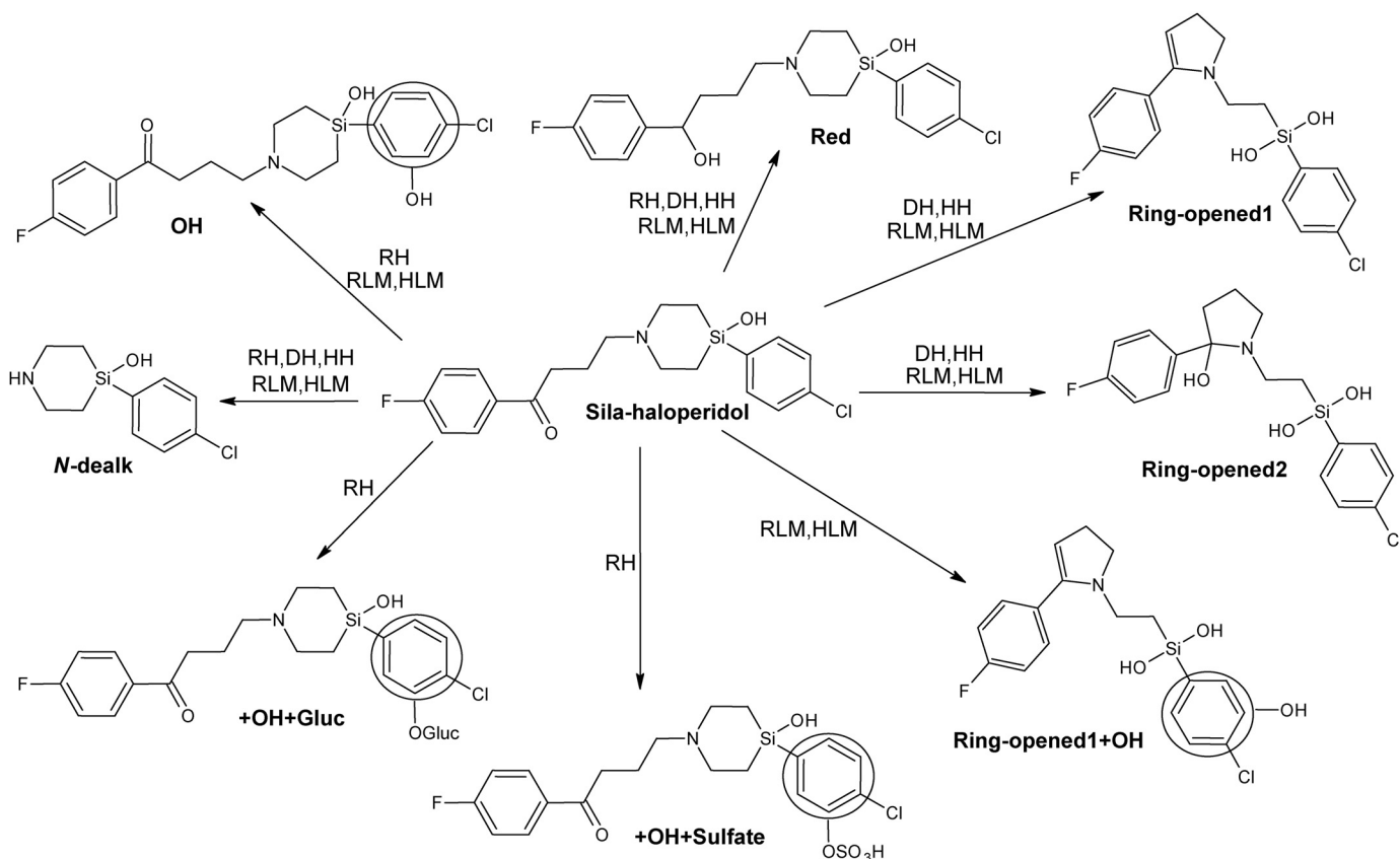
FIG. 3. Proposed overall metabolism of sila-haloperidol in HLMs, RLMs, and hepatocytes (HH, human; DH, dog; RH, rat).
