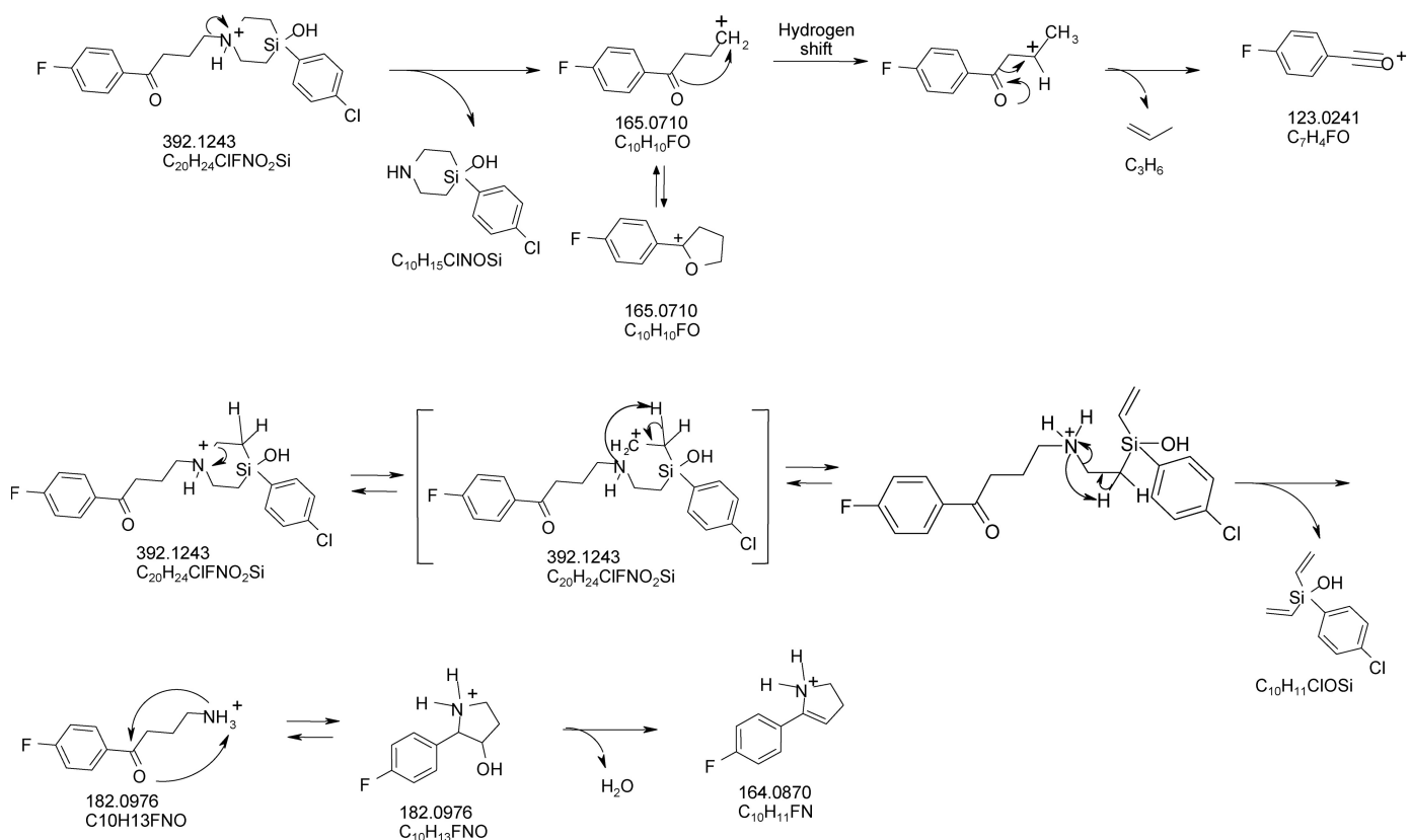
FIG. 5. Proposed fragmentation pathways of sila-haloperidol.
