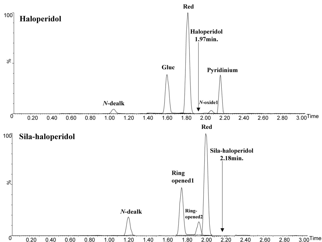
FIG. 8. Metabolism of haloperidol and sila-haloperidol, respectively, by human hepatocytes. Extracted ion chromatograms of m/z 212, 552, 378, 392, and 354 for haloperidol and m/z 228, 364, 382, and 394 for sila-haloperidol. The retention times of haloperidol and sila-haloperidol are marked in the different chromatograms.
