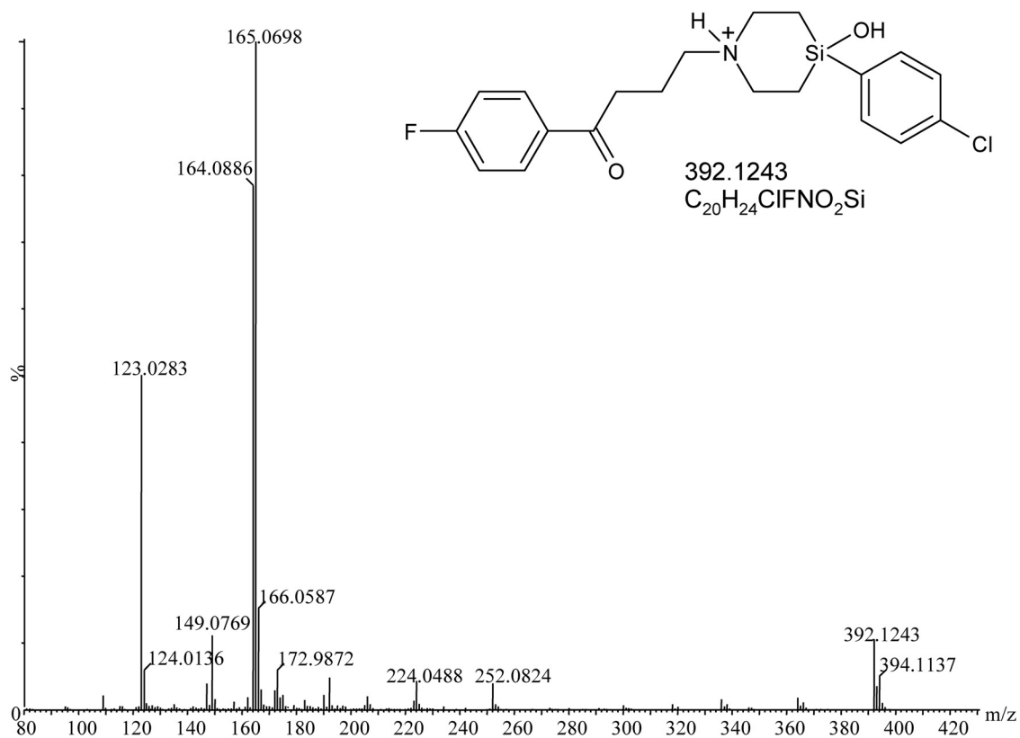
FIG. 4. Product ion spectrum of sila-haloperidol.
