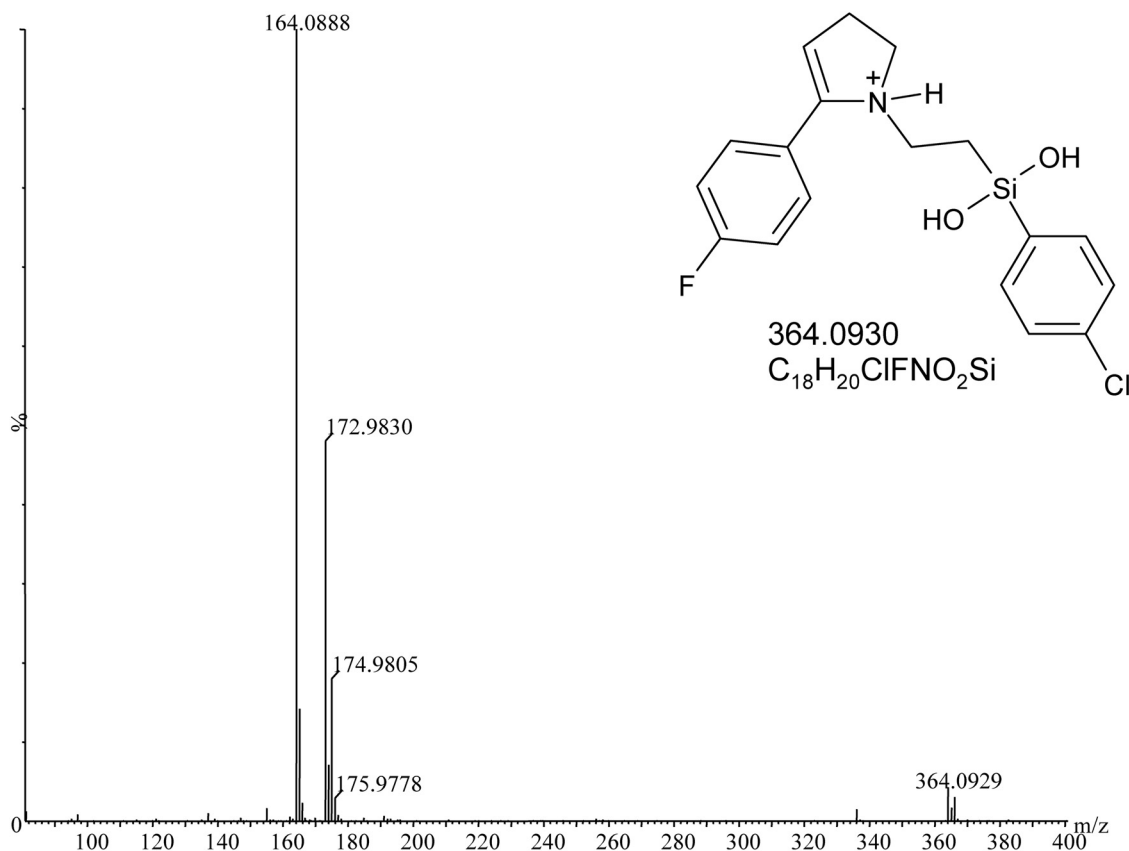
FIG. 6. The product ion spectrum of the ring-opened1 metabolite of sila-haloperidol.
