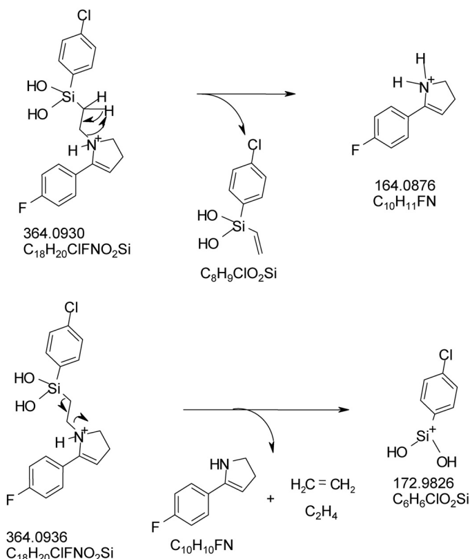
FIG. 7. Proposed fragmentation pathways of the ring-opened1 metabolite of sila-haloperidol.
