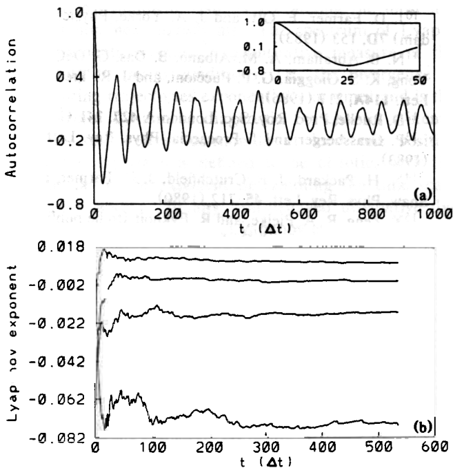
FIG. 1. (a) Autocorrelation function, and (b) convergence of Lyapunov exponents for the Mackey-Glass equations with parameters a=0.2, b=0.1, c=10 , and T=23 , and other parameters as described in the text. The inset graph is a magnification of the region close to the origin in (a).
