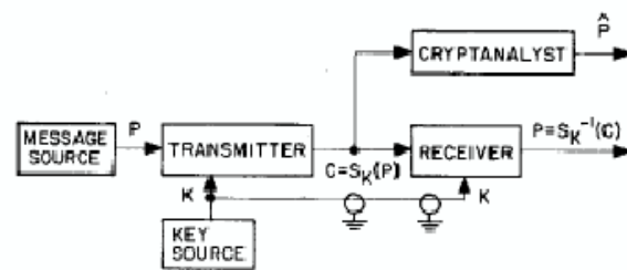
Figure 1: Flow of informatrion in conventional cryptographic system.
