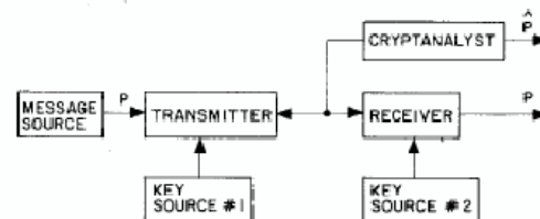
Figure 2: Flow of information in public key system.
