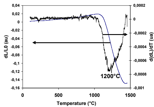
Fig 6. \Delta L/L_0 and differential curves as a function of the heating temperature.
