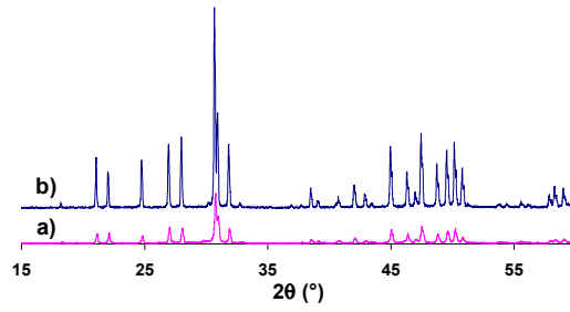
Fig 3. X-ray diffraction pattern (Cu-K \alpha ) of La 9.33 Si 6 O 26 oxides powders heat-treated at 1000°C a) and ceramics heat-treated at 1500°C b).
