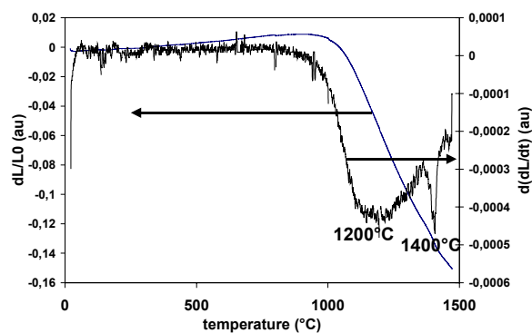
Fig 2. \Delta L/L_0 and differential curves as a function of the heating temperature.
