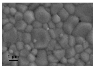
Fig.7. Scanning Electron Micrograph of \text{La}_{9.33}\text{Si}_6\text{O}_{26} ceramics with a sintered density of 92%
