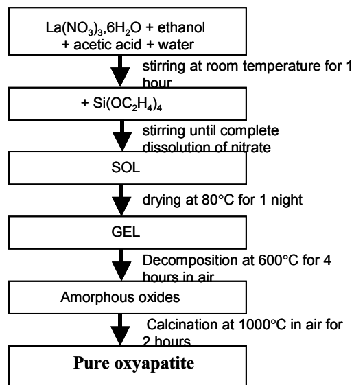
Fig. 1. flow chart of preparation of for \text{La}_{9,33}\text{Si}_6\text{O}_{26} powders.
