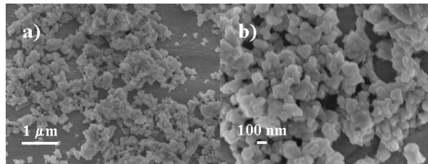
Fig 5. SEM-FEG feature of \text{La}_{9.33}\text{Si}_6\text{O}_{26} powders calcined at 1000^\circ\text{C} and attrition milling.
