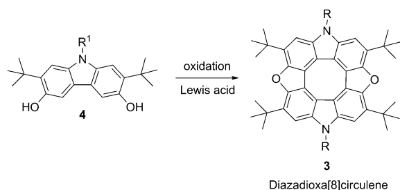
Scheme 3. Synthesis of diazadioxa[8]circulene ( 3 ). R = propyl ( 3 Pro ) or benzyl ( 3 Bn ). Conditions: oxidant (chloranil or DDO), Lewis acid ( \text{BF}_3\cdot\text{OEt}_2 , \text{FeCl}_3 , or \text{AlCl}_3 ), \text{CH}_2\text{Cl}_2 , yield: 71–85%.
