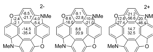
Figure 4. NICS(0) and NICS(1) zz (lower numbers) values calculated for diazadioxo[8]circulene ( 3 Me ). For comparison, the same values for tetraoxa[8]circulene ( 1 ) and azatrioxa[8]circulene ( 2 ) are given in the Supporting Information.
