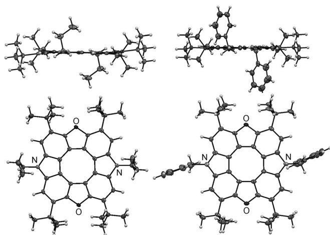
Figure 2. Single-crystal X-ray structure of 3 Pro (left) and 3 Bn (right). The top pictures show a side-view illustrating the planarity of the diazadioxa[8]circulenes and the bottom images show the front view of the structures.
