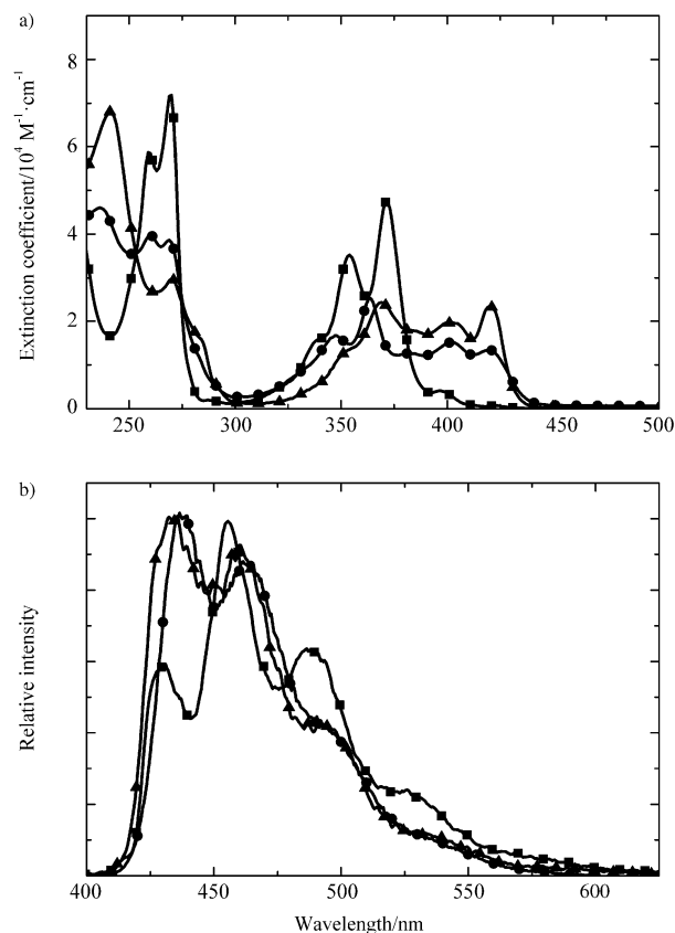
Figure 3. a) UV/Vis and b) fluorescence spectra of 1 ( \blacksquare ; 0N), 2 Pro ( \bullet ; 1N), and 3 Pro ( \blacktriangle ; 2N) recorded in \text{CH}_2\text{Cl}_2 .
