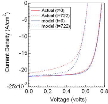
Figure 10 Voltage-dependent collection
