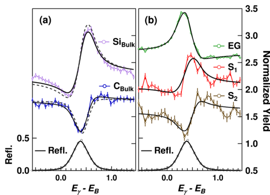
FIG. 3 (color online). XSW results for (a) near-surface bulk and (b) surface species corresponding to XPS components in Figs. 2(c) and 2(d). Measured (gray circles) and fitted (black) reflectivity from the SiC(0006) Bragg peak are plotted vs energy offset from the geometrical Bragg condition ( E_B = 2450 eV). Normalized yields and best-fit results (black) are offset for clarity, and simulated yields for ideal SiC bulk are in dashed black.
