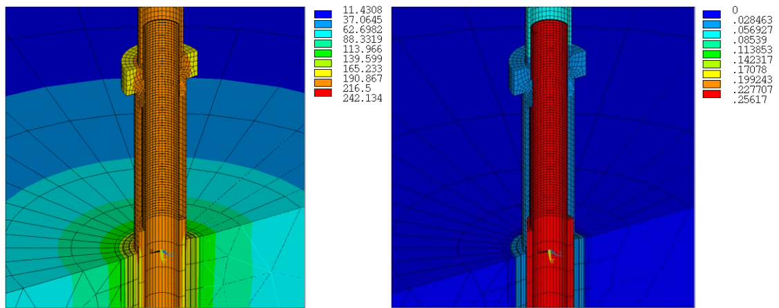
Figure 7: Left: temperature distribution of the wellhead three months after discharge (°C). Right: axial displacement of the wellhead (meters) after going through the load history that is listed in Table 4 (180° symmetry expansion of the wellhead of model i).
