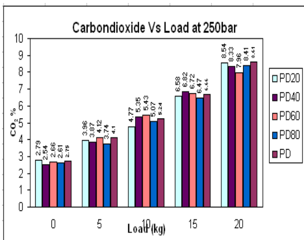
Fig. 11 Carbon dioxide V/s Load graph with Blends of Plastic Diesel with Diesel, at 250 bar Pressure
