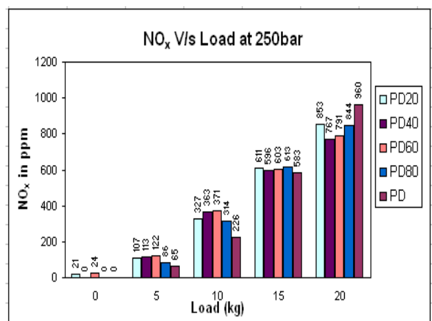
Fig. 8 Nitric Oxide V/s Load graph with Blends of Plastic Diesel with Diesel, at 250bar Pressure
