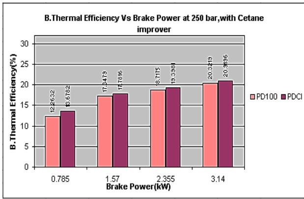
Fig.14 Brake Thermal Efficiency V/s Brake Power graph with blends of with blends of Plastic Diesel with Diesel, at 250 bar Pressure
