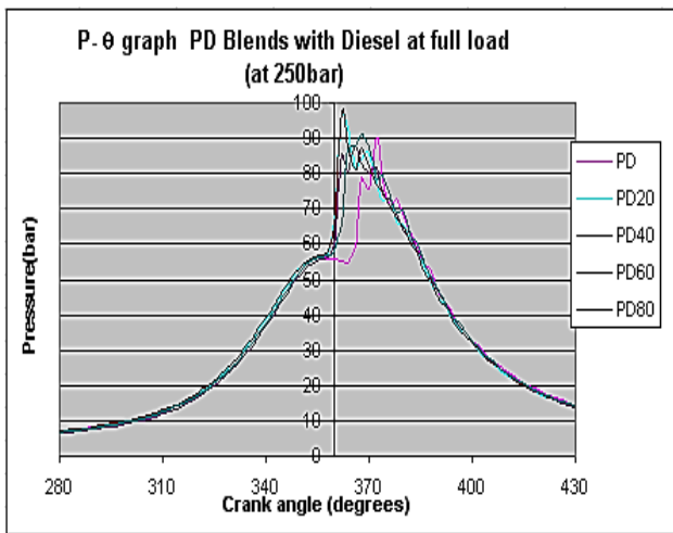
Fig. 5 P-θ Graph at full load with Blends of Plastic Diesel with Diesel, at 250bar Pressure
