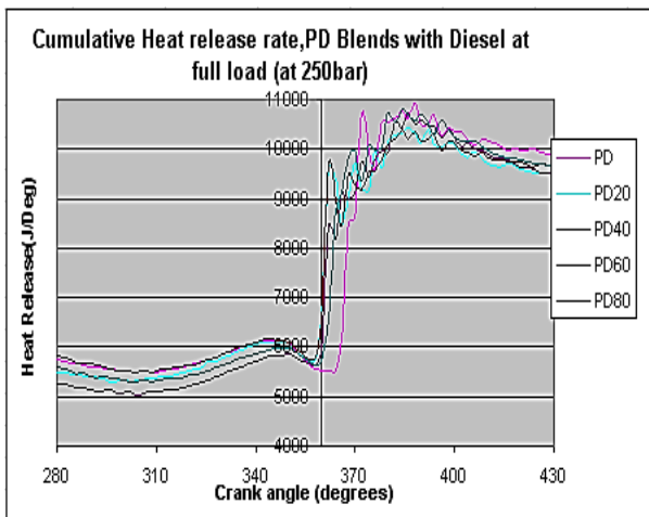
Fig. 6 P-θ Graph at full load with Blends of Plastic Diesel with Diesel, at 250bar Pressure
