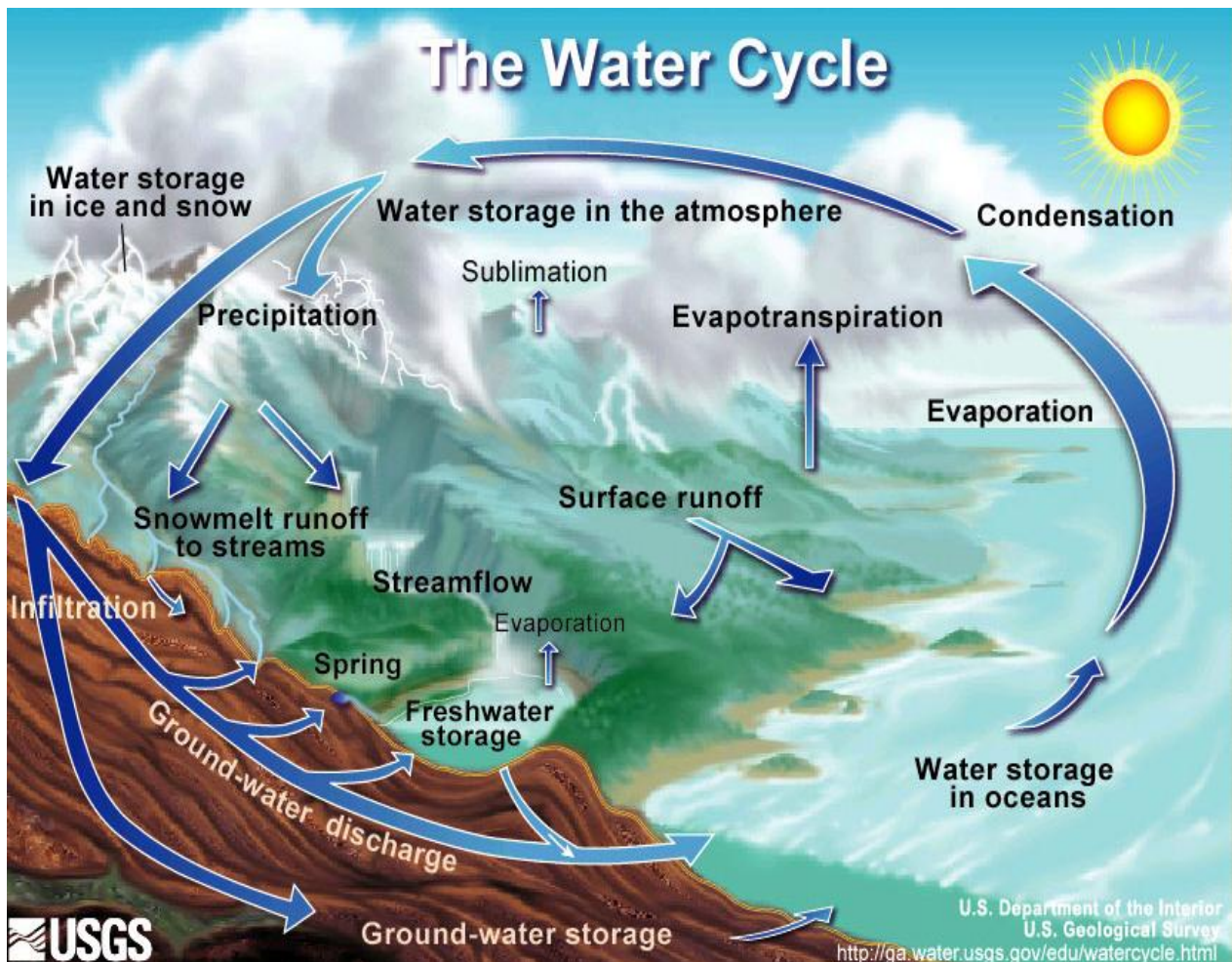
Figure 1. Hydrologic cycle.
