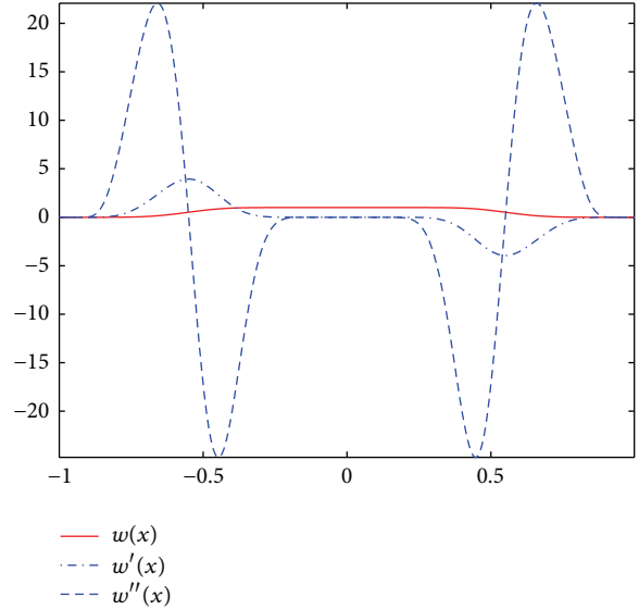
FIGURE 4: We show w(x) = \sin((\pi/2)(e^{-c/x}/(e^{-c/x} + e^{-c/(1-x)}))) , dw(x)/dx , and d^2w(x)/dx^2 where c = 1.57 .
