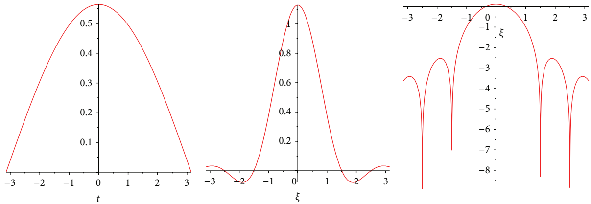
FIGURE 1: The figure shows window function g(t) = \sqrt{1/\pi} \cos(t/2) \mathbf{1}_{[-\pi, \pi]}(t) , its Fourier transform \hat{g} , and \log(|\hat{g}|) .
