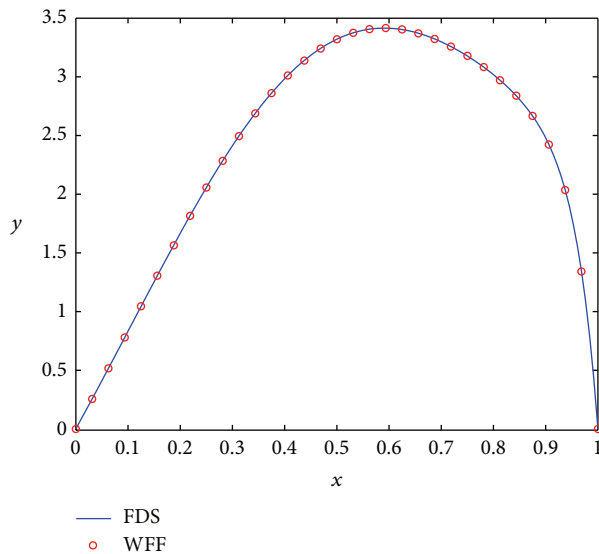
FIGURE 7: Solution of the BVP: using windowed Fourier frames and using a standard finite difference scheme.
