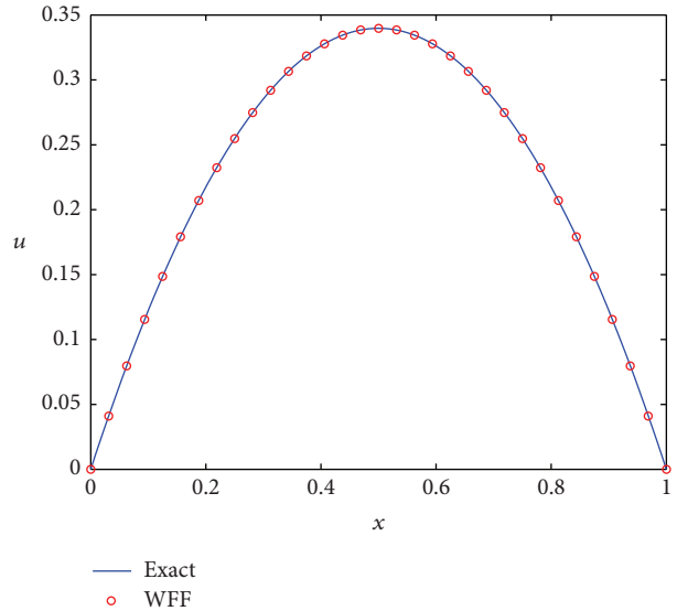
FIGURE 5: Solution of the BVP: using windowed Fourier frames.
