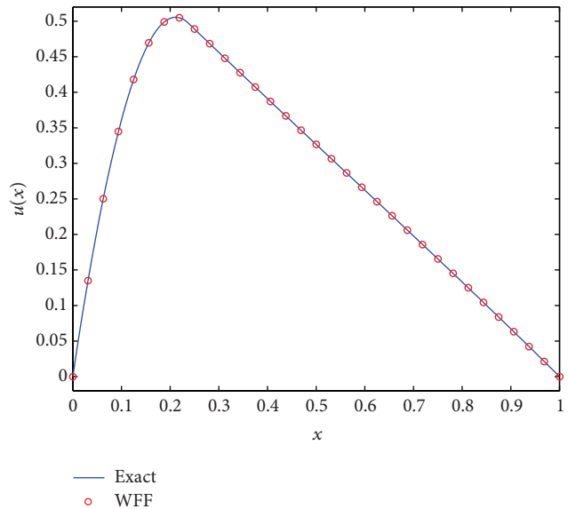
FIGURE 6: Solution of the BVP: using windowed Fourier frames.
