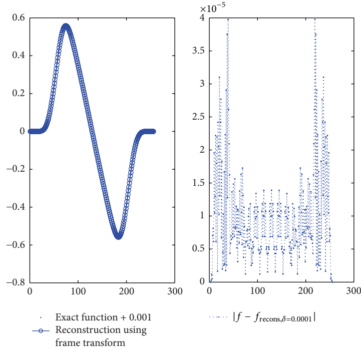
FIGURE 3: This figure shows the original function f and recovered function from the frame coefficients ( |C_{j,k}| > \delta = 10^{-4} ) and the error we made with such an approximation.
