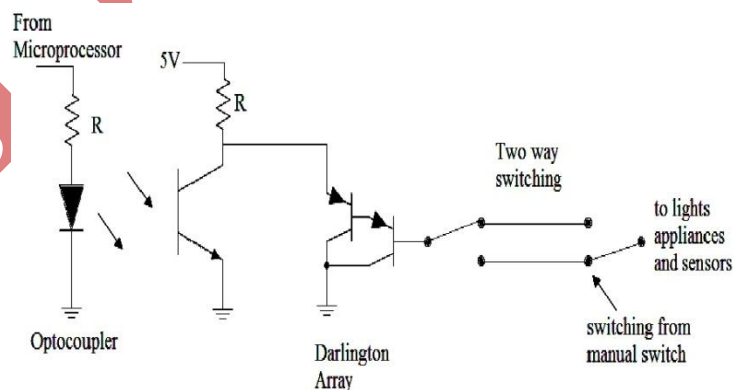
Fig. 3 Switching from low voltage to high voltage
