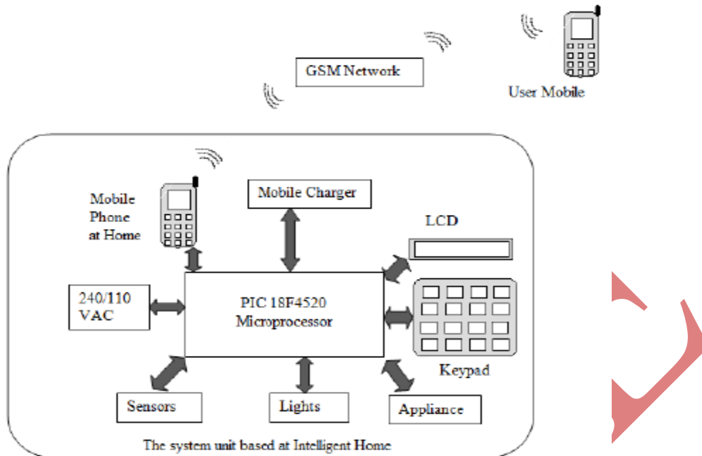
Fig. 1 Architecture of Intelligent Home system
