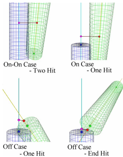
Fig. 6 Cylinder testing
