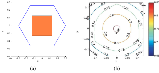
Fig. 6. (a) Workspace cross section at z = z_c ; (b) contour plot of the inverse condition number of J at z = z_c .
