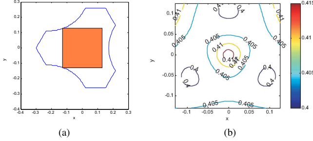
Fig. 7. (a) Workspace cross section at z = z_c + l^* ; (b) contour plot of the inverse condition number of J at z = z_c + l^* .
