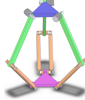
Fig. 4. A CAD model of the resulting Delta robot
