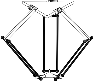
Fig. 2. Architecture of the Delta robot
