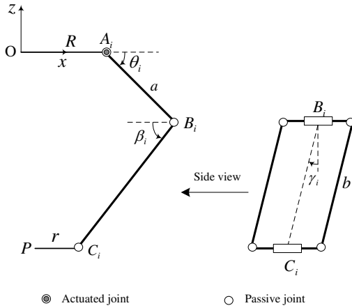
Fig. 3. The i -th subchain of the Delta robot
