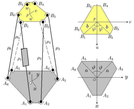
Fig. 8. A schematic for the Gough-Stewart platform
