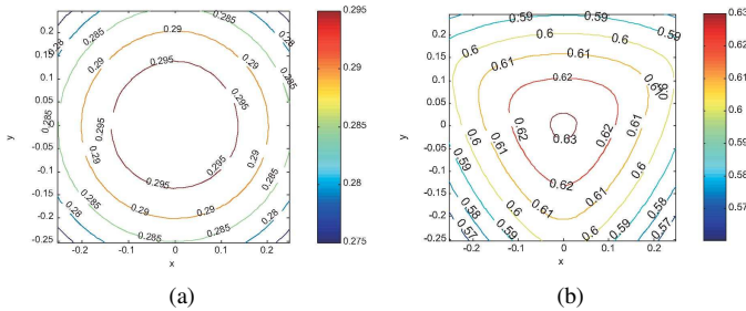
Fig. 11. Contour plots of (a) \kappa(J_z) and (b) \kappa(J_\Psi) at z = z_c and \eta = 0 .
