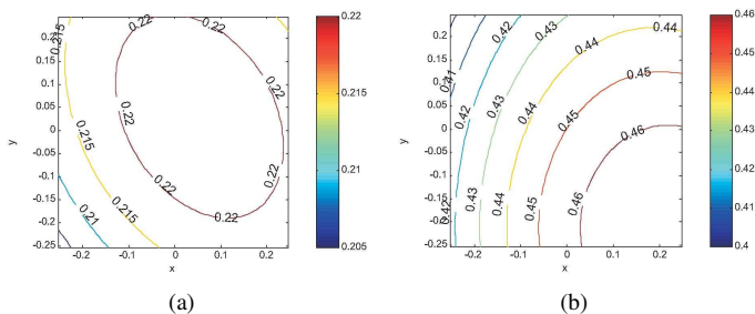
Fig. 12. Contour plots of (a) \kappa(J_z) and (b) \kappa(J_\Psi) at z = z_c + l^* and \eta = -30^\circ about the direction (-\frac{\sqrt{3}}{2}, \frac{1}{2}, 0) .
