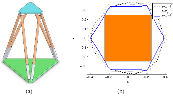
Fig. 10. (a) A scaled model of the resulting Gough-Stewart platform; (b) workspace cross sections of the optimal manipulator.
