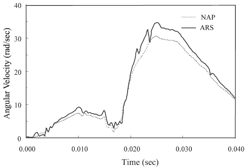
Fig. 11a. Non-contact test, resultant angular velocity.
