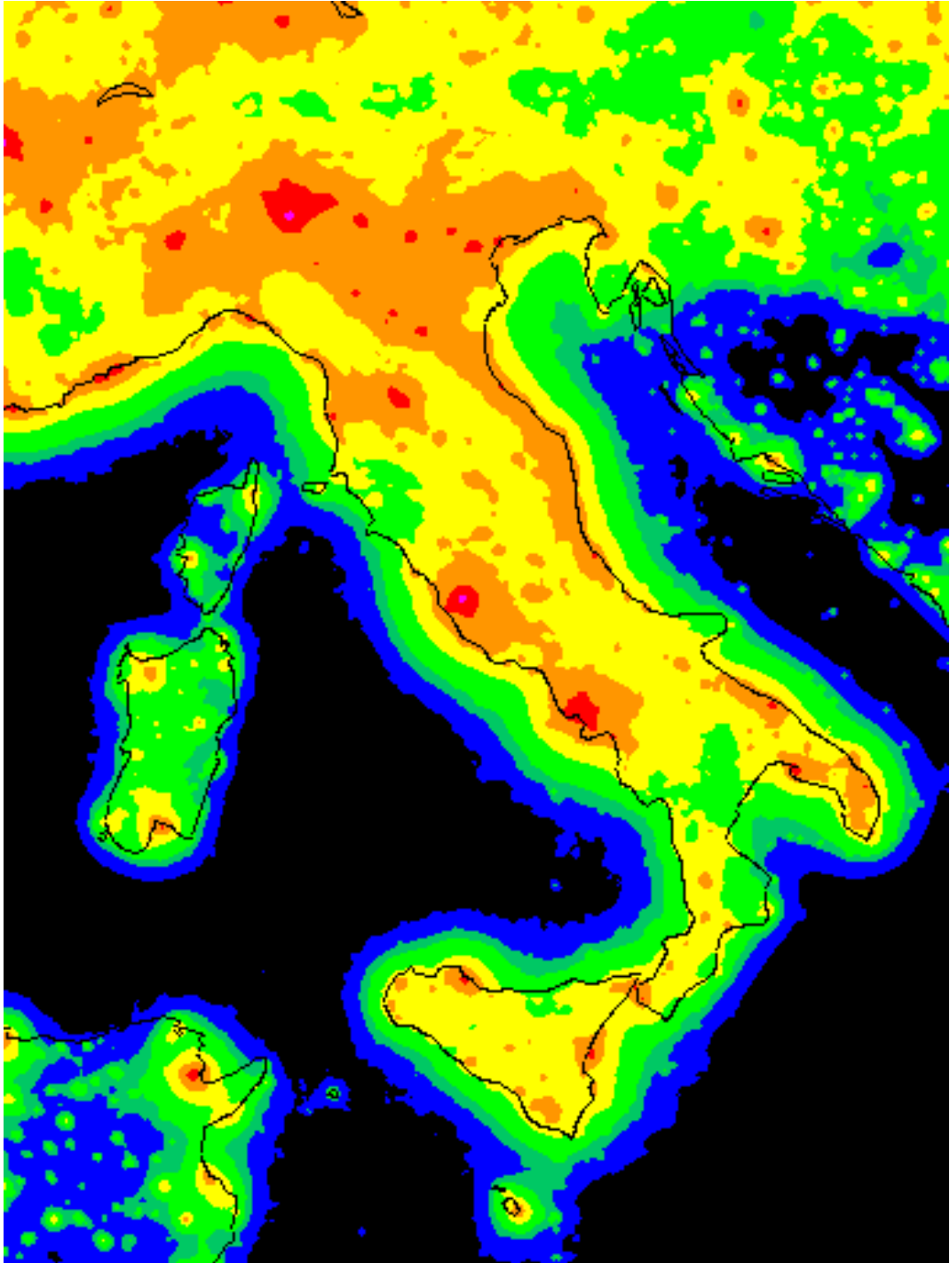
Fig. 2. Map of the artificial sky brightness in Italy in 1998. Levels correspond respectively to <0.05 , 0.05-0.15 , 0.15-0.35 , 0.35-1.1 , 1.1-3 , 3-10 , 10-30 , >30 times the natural sky brightness. Contours of Italy are only an indication.
