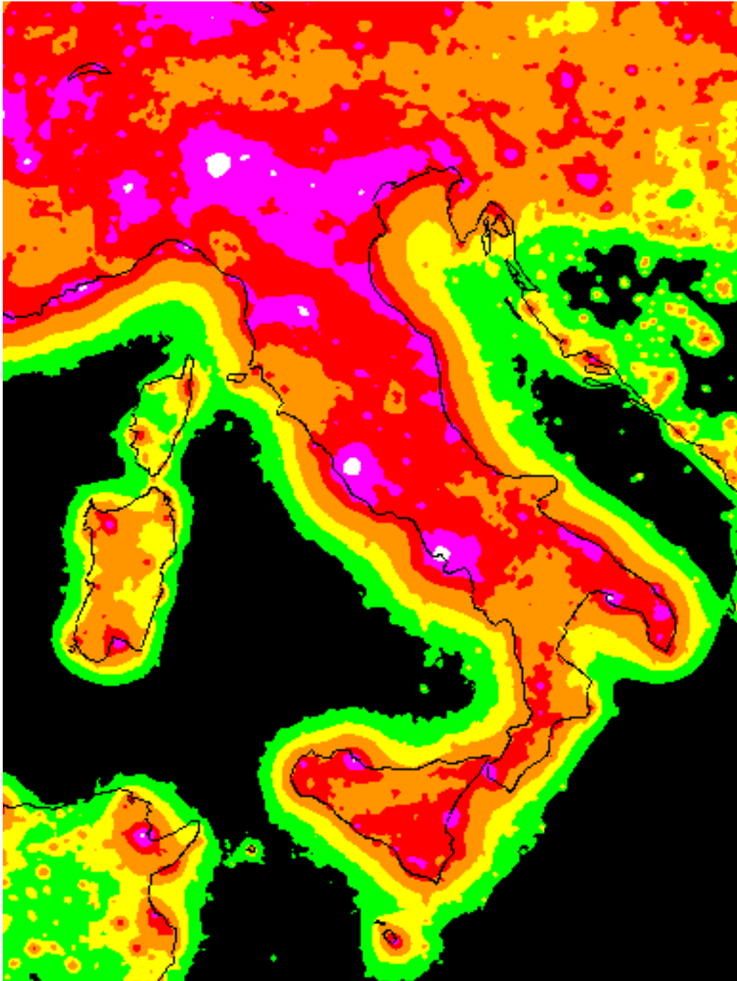
Fig. 3. Map of the artificial sky brightness in Italy extrapolated to the year 2025. Levels correspond respectively to <0.35 , 0.35-1.1 , 1.1-3 , 3-10 , 10-30 , 30-100 , >100 times the natural sky brightness. Contours of Italy are only an indication.
