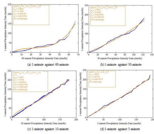
Fig. 5: Graphs and the curve-fitting process execute by the software.
