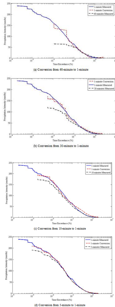
Fig. 6: Comparison between the results of the conversion technique and the of measurements data of 1-minute integration time.
