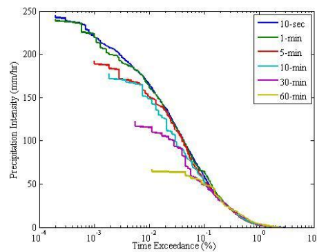
Fig. 3: Plotted graphs for precipitation intensity statistics obtained
