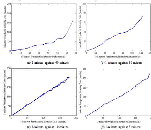
Fig. 4: Plots of the 1-minute precipitation intensity statistics data against the desired precipitation intensity statistics data.
