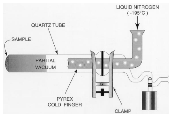
Fig. 1. MOD breadboard sublimation apparatus. The apparatus is made out of a pyrex cold finger and a quartz tube. The sample is placed on the bottom of the quartz tube before it is connected to the pyrex cold finger and sealed. The whole assembly is connected to a vacuum line until the pressure is less than 500–600 mTorr. After that, the sublimation assembly is inserted into a heater. Heating time is usually 1–5 min at 450°C. Liquid nitrogen has to be supplied during the heating to cool the cold finger.
