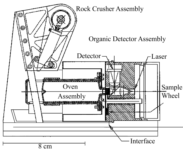
Fig. 4. MOD prototype design. The total mass of the MOD, including the rock crusher is 2300 g. The sample (0.1–1 g) can be introduced through the introduction port of the rock crusher (in case of solid cores) or directly into the sublimation zone inlet. Drawing provided by C. LaBaw, NASA-JPL.
