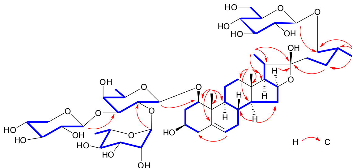
Figure 2. Selected COSY (—) and HMBC (—) correlations of compound 1 .
