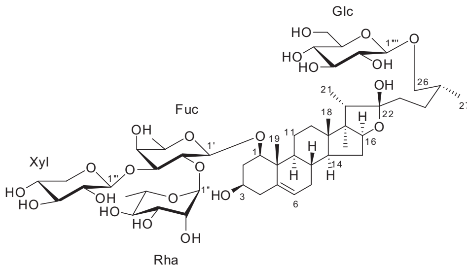
Figure 1. Chemical structure of ophiopogonin T (1). Xyl: xylose; Rha: rhamnose; Fuc: fucose; Glc: glucose.
