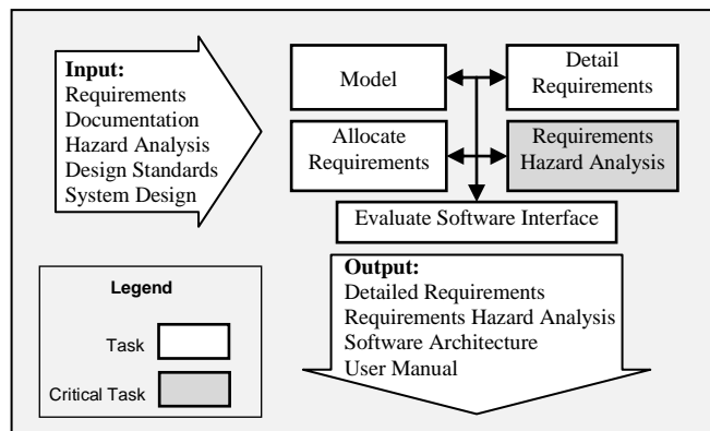
Figure 6. Analysis (stage process pattern)
