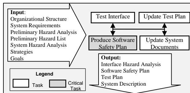
Figure 14. Interface Hazard Analysis (stage process pattern)
