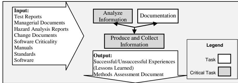
Figure 16. Assessment (stage process pattern)
