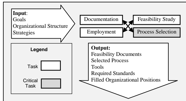
Figure 3. Establish Infrastructure (stage process pattern)
