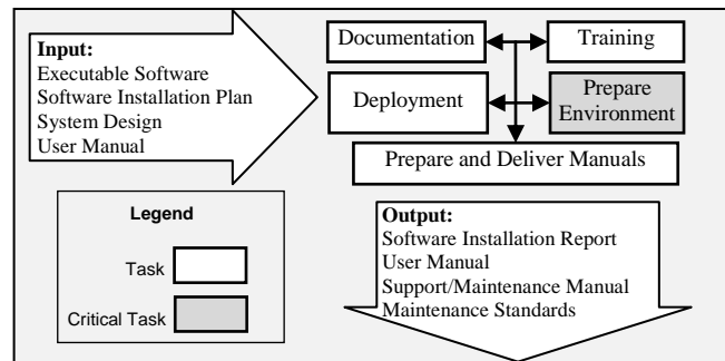
Figure 13. Deploy (stage process pattern)
