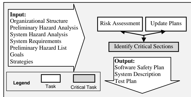
Figure 4. Hazard Analysis – Initiation (stage process pattern)
