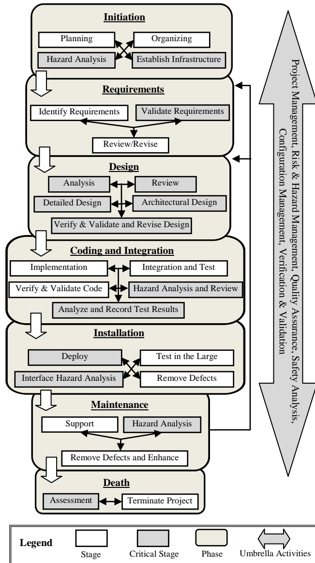
Figure 2. HISDP and its constituent Stage process patterns
