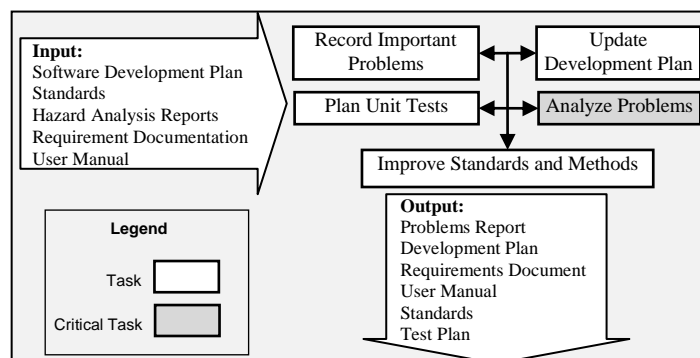
Figure 10. Review (stage process pattern)
