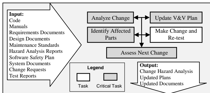
Figure 15. Hazard Analysis – Maintenance (stage process pattern)
