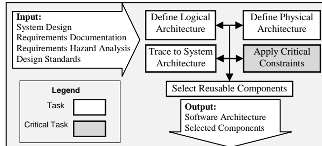
Figure 7. Architectural Design (stage process pattern)
