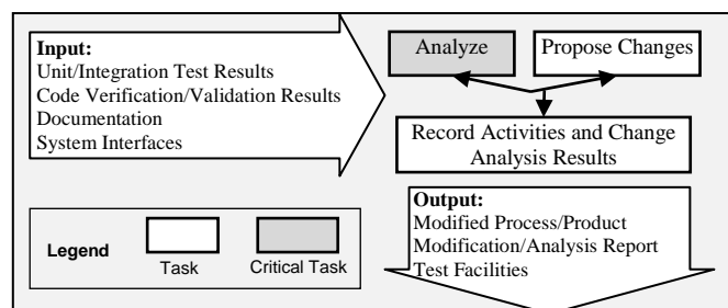
Figure 12. Hazard Analysis and Review (stage process pattern)
