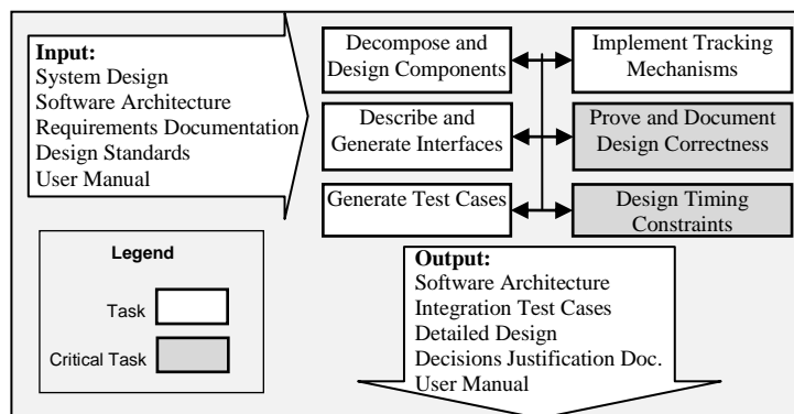
Figure 8. Detailed Design (stage process pattern)
