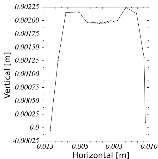
Figure 3: Dynamic aperture, calculated at the injection, obtained after splitting the sextupoles into 15 independent families
