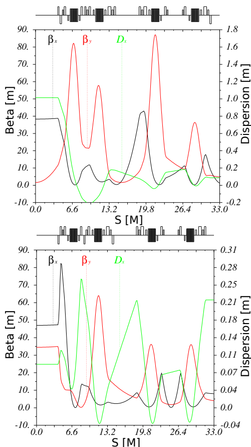
Figure 2: Two different solutions for the full arc. The one on the top is workable up to 2.4 GeV, the one on the bottom up to 2.0 GeV
