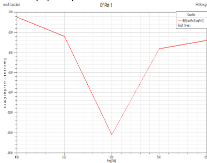
Fig 3- Return loss for proposed system
