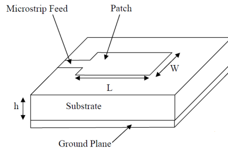
FIG 1 – MICROSTRIP PATCH ANTENNA
