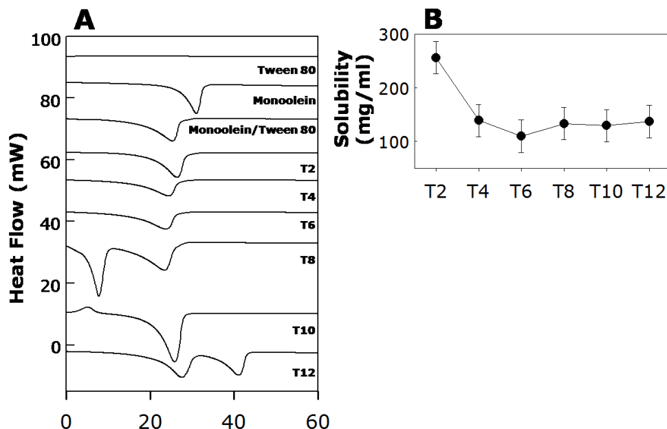
Fig. 3. A) Heating thermograms obtained from the formulations prepared with different triglycerides (T2 ~ T12, in Table 2), Tween 80, monoolein and monoolein/Tween 80 (55.0:16.5 by weight). The concentration of paclitaxel was 1 % (w/w) in all formulations. B) Solubility of paclitaxel in the formulations containing monoolein, triglyceride and Tween 80 at 55.0:27.5:16.5 by weight at 37 °C.
