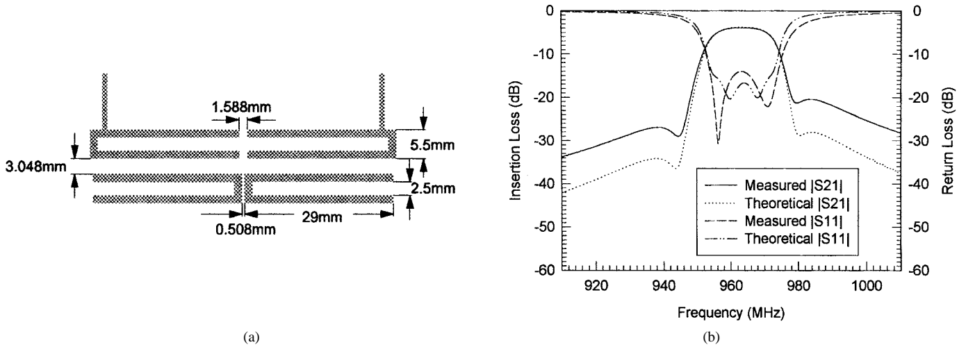
Fig. 4. (a) Layout of the four-pole cross-coupled hairpin-resonator bandpass filter with 2.07% fractional bandwidth at 965 MHz on an RT/Duroid substrate (not shown) with \epsilon_r = 10.8 and a thickness h = 1.27 mm. The resonators are almost identical for this narrow-band filter. (b) Measured and theoretical responses of the filter.
