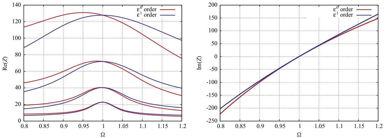
Fig. 10. Comparison of the impedance obtained from the y_0 and y_0 + \epsilon y_1 approximations for 100 dB, 110 dB, 120 dB and 130 dB. Same configuration as in Fig. 5.
