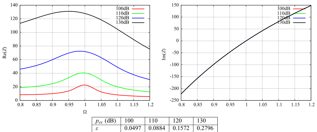
Fig. 5. Real and imaginary parts of impedance Z for a Helmholtz resonator as a function of nondimensional frequency at different driving amplitudes. The realistic configuration that is chosen corresponds with S_n/S_b = 0.05 , r = 0.2 , \omega_0/2\pi = 1447 Hz, L = 0.035 m, \ell = 0.002 m.
