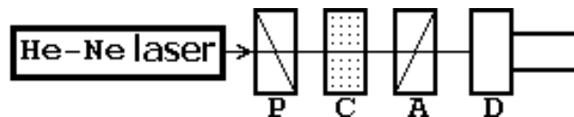
Fig.2. He-Ne laser (633nm), P is the polarizer, C is liquid crystal cell, A is the analyzer, D is the photodetector.
