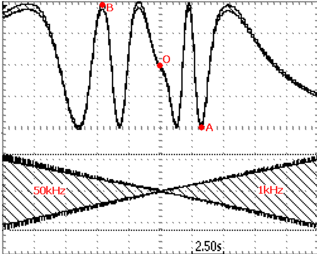
Fig.8. The photodiode signal shows dynamics of phase shift caused by transition between quasi-planar states B and quasi-homeotropic state A. In state O applied voltage is 0V.
