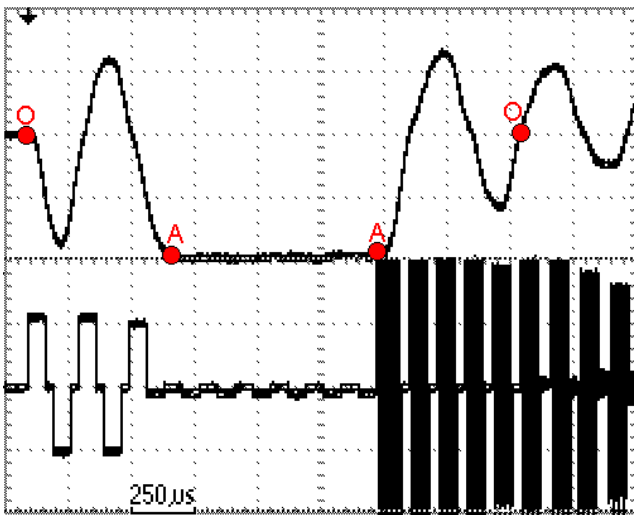
Fig.9. In optical retardation similar to scenario on Fig. 7 “the pause” of the switching process was performed in state A.
