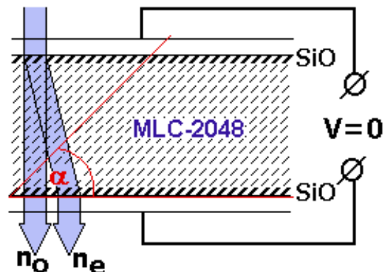
Fig.1 Initial tilted orientation of dual frequency nematic cell.
