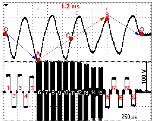
Fig.7. Fast optical retardation switching with \Delta L = 10 \Delta L \approx 1.6 \mu m in \tau_{A \rightarrow B} \approx 1.2 ms , where A and B are states of the dual frequency liquid crystal in Fig.8.
