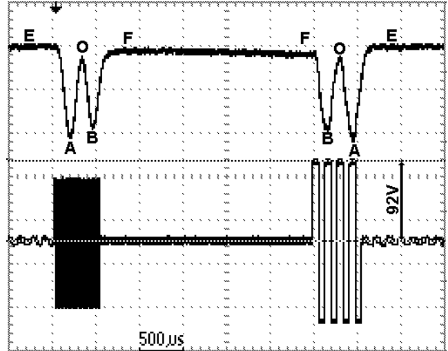
Fig.6. One cycle of fast switching between states E and F in Fig.3, switching amplitude of the optical retardation is \Delta L \approx 1.266 \mu m .
