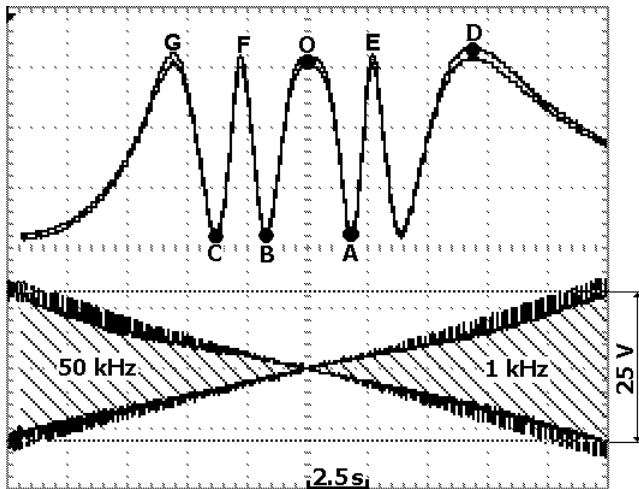
Fig.3. Optical transmission of 12 \mu\text{m} thick nematic cell (top trace) registered by the photodetector D as the function of applied voltage (bottom trace) at 50 kHz (left part) and 1 kHz (right part).
