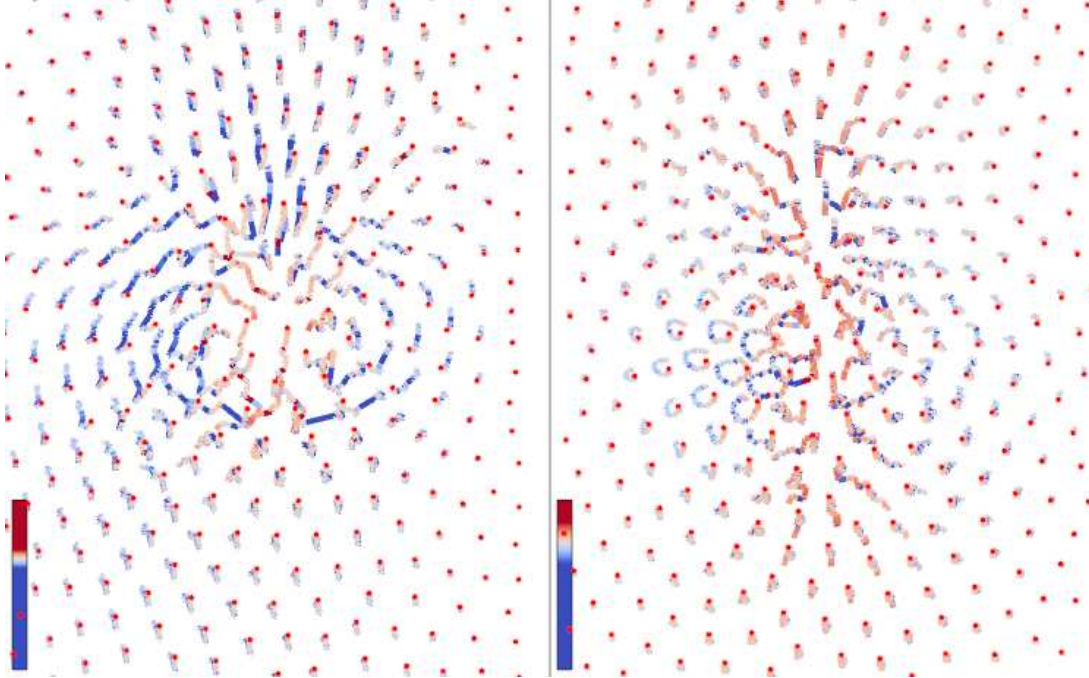
Figure 5: Bubble paths, coloured by vertical velocity, near a sedimenting ellipse which has its long axis horizontal (left) or vertical (right). The colour scale is the same in each case, symmetric about zero velocity, although the range of velocities is larger in the horizontal case. The initial position of each bubble is shown with a red dot. Only in the vertical case, when the ellipse moves more quickly, do the bubbles describe loops.
