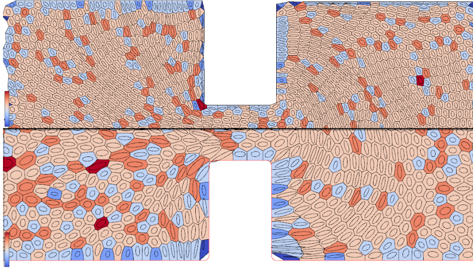
Figure 7: A photograph of an experiment in which a foam flows through a constriction can be reconstructed in Surface Evolver [12], and then visualized in FoamVis. Here we compare such an experiment (top) with a simulation (bottom), as described in §3.2. Each bubble is coloured by its number of sides, and contains an ellipse (a texture tensor) indicating the direction and magnitude of the local strain. Note that there are many more bubbles in the experiment, and that the strain is lower, presumably because of the finite liquid fraction.
