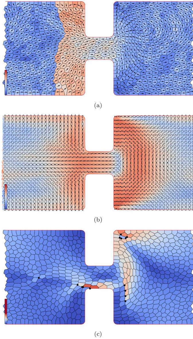
Figure 2: Flow of a foam through a 4:1:4 constriction from left to right. (a) Bubbles coloured by instantaneous pressure, with their direction of motion (velocity vectors with equal length) indicated. Note the region of high pressure just upstream of the constriction, and the apparent vortex in one of the upstream corners. (b) A rolling average of the texture tensor (ellipses), with pixels coloured by the average of its largest eigenvalue, indicating the local strain. The foam is isotropic far from the constriction, but the bubbles are elongated parallel and perpendicular to the direction of flow up- and downstream respectively. (c) Bubbles with large instantaneous velocities appear to correlate with the position of TIs (black dots); it is also apparent that TIs often occur in avalanches, and that their effect on bubble motion is extensive.
