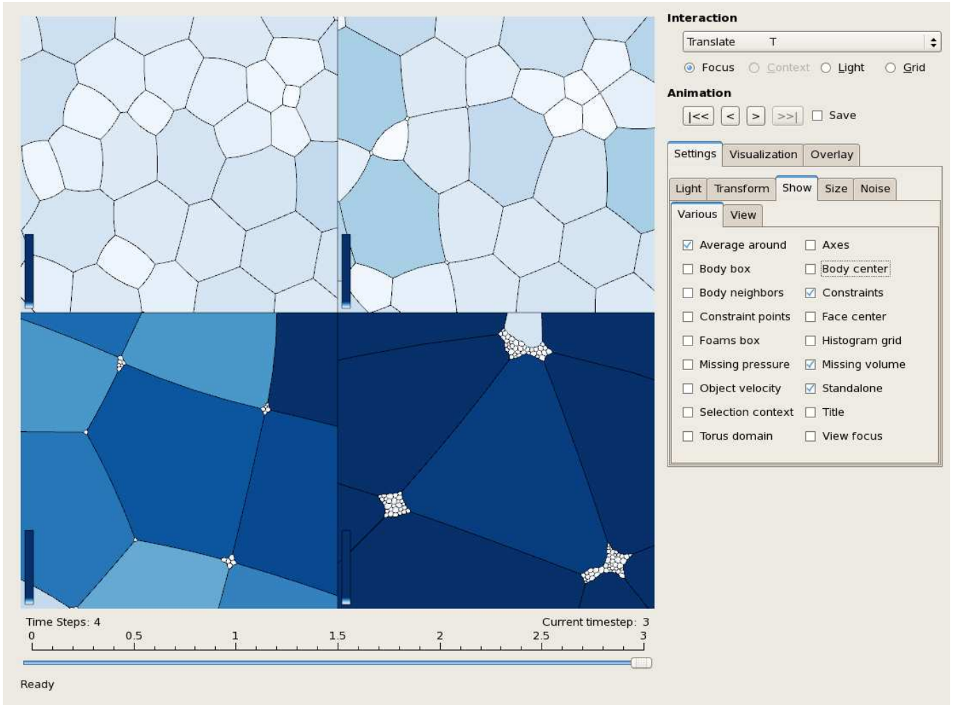
Figure 1: A screenshot of FoamVis for a simulation in which a foam containing a mixture of two gases undergoes diffusion-driven coarsening. The foam is shown at timesteps 10^2 , 10^3 , 10^4 and 10^5 . Bubbles are coloured by area, and the same bubble is kept at the centre of the field of view. The foam gradually segregates into a few large bubbles with equal pressure, with many smaller bubbles of roughly equal size clustered around their vertices.
