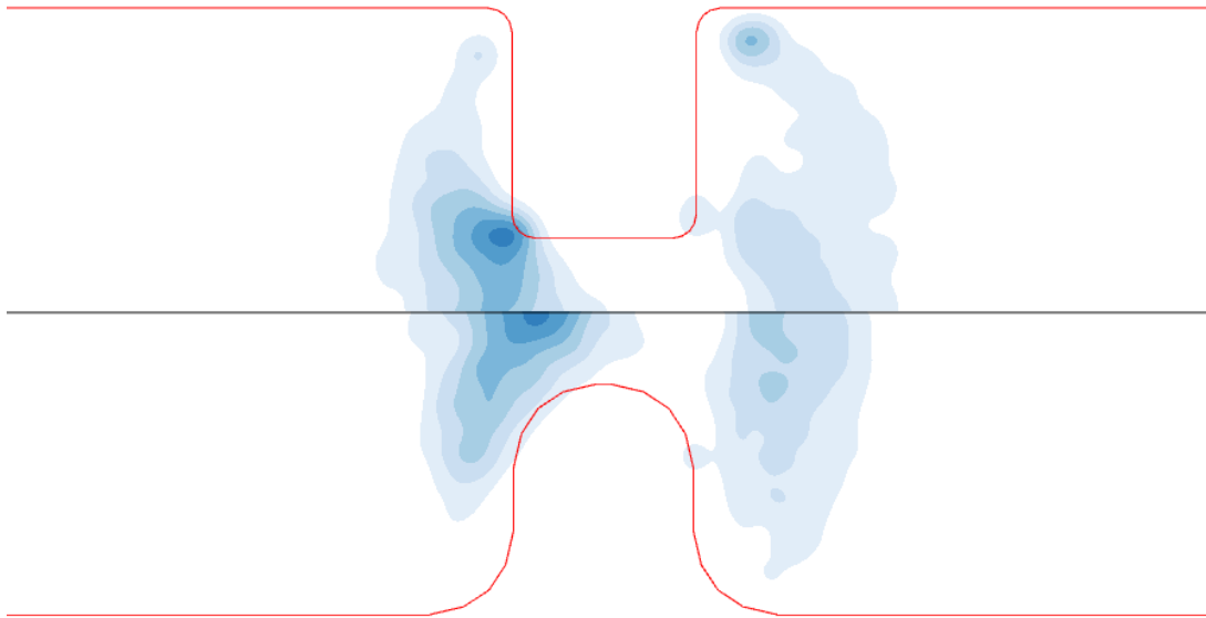
Figure 3: Flow of a foam through a 4:1:4 constriction, showing a smoothed profile of T1 density. The cumulative distribution of T1s changes when the corners of the constriction are either sharp (top) or rounded (bottom). It is apparent that there are more T1s upstream than downstream, and that for the case of a sharp corner most T1s occur close to the corners and the maximum in T1 intensity is shifted upstream.
