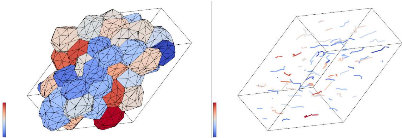
Figure 6: Quasistatic simple shear of a polydisperse dry three-dimensional foam of 65 bubbles, with periodic boundary conditions (shown as a parallelepiped, cf. [17]). Using the multiple views feature, FoamVis animates the foam on the left and shows the corresponding bubble paths on the right. Bubbles and paths are coloured by bubble volume. Sudden changes in path direction are a result of T1s.
