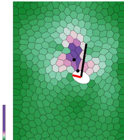
Figure 4: The instantaneous network (black line) and pressure (red line) forces on an ellipse sedimenting under its own weight. The torque due to these forces is not shown. The bubbles are coloured by the magnitude of the velocity of their centres, and the position of T1s is shown as black dots.
