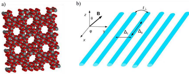
Fig. 1. Structure of (a) a porous zeolite with periodic channels, and (b) the corresponding model for the quasi-1D superconducting wires on a plane.
