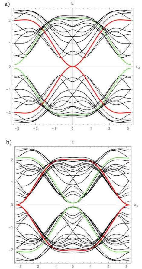
Fig. 2. The energy spectrum of quasi-1D superconductor as a function of k_x in the non-trivial topological phase ( \nu = 1 ) for (a) \Delta_0 > 0 with a zero-energy state (red curves) at the center of the Brillouin zone and (b) \Delta_0 < 0 with a zero energy state (red curves) at the boundaries of the Brillouin zone. The parameters are chosen in the unit of the band width 2t_{\parallel} = 1 . In both cases |\Delta_0| = 0.5 \times 2t_{\parallel} we choose, t_{\perp} = 0.2 \times 2t_{\parallel} and \alpha = 0.6 \times 2t_{\parallel} .
