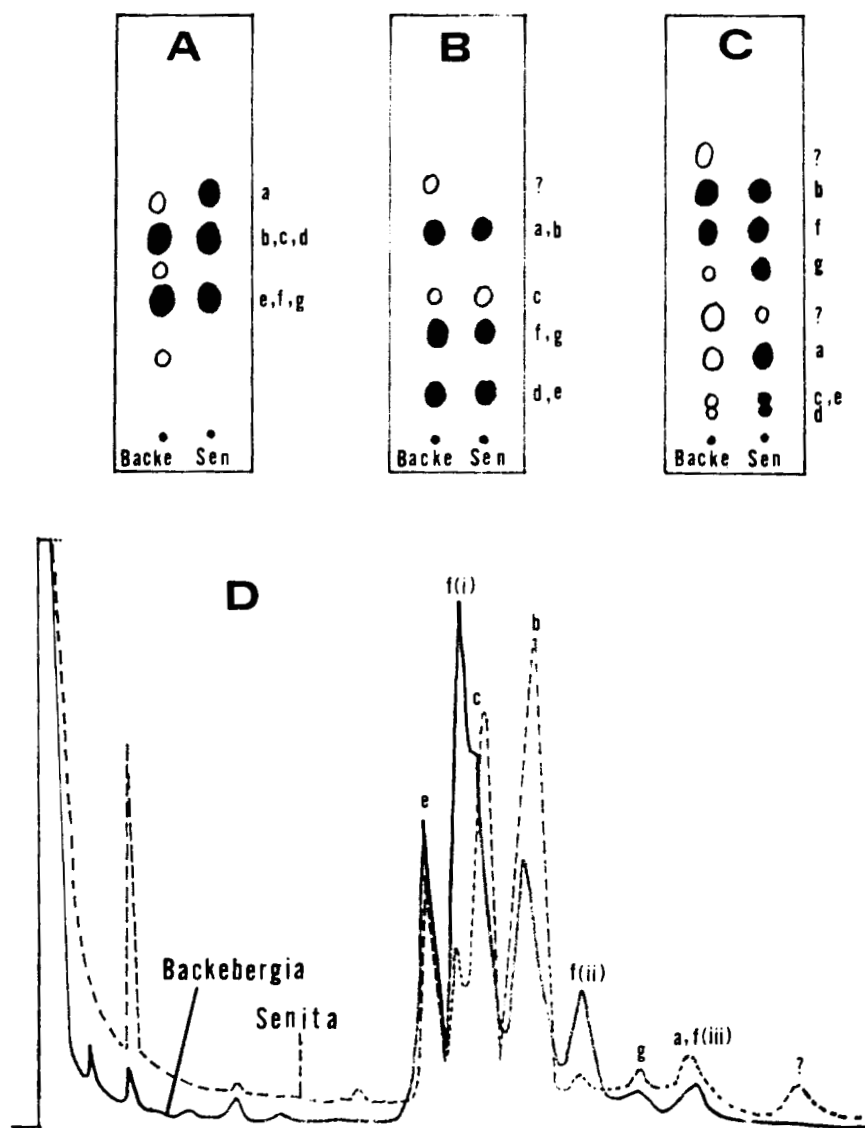
Fig. 1. Chromatographic comparisons of Backebergia militaris and senita cactus non-saponifiable fractions. TLC: A. 60/40 hexane-EtOAc, Sigel plate. B. 95/5 \text{CHCl}_3 - \text{Me}_2\text{CO} , \text{AgNO}_3 Plate, 2 X. C. \text{CH}_2\text{Cl}_2 , \text{AgNO}_3 plate, 2 X, acetates. GC: D. 5% OV-101, 270°. a) lup-20(22)-en-3 \beta -ol, b) 4 \alpha -methylcholest-7-en-3 \beta -ol, c) 4 \alpha -methylcholesta-8,14-dien-3 \beta -ol, d) 4 \alpha -methylergosta-7,24(28)-dien-3 \beta -ol, e) cholesta-8,14-dien-3 \beta -ol, f) (i) cholest-7-en-3 \beta -ol, (ii) campest-7-en-3 \beta -ol, (iii) stigmast-7-en-3 \beta -ol, g) stigmasta-7,22-dien-3 \beta -ol.
