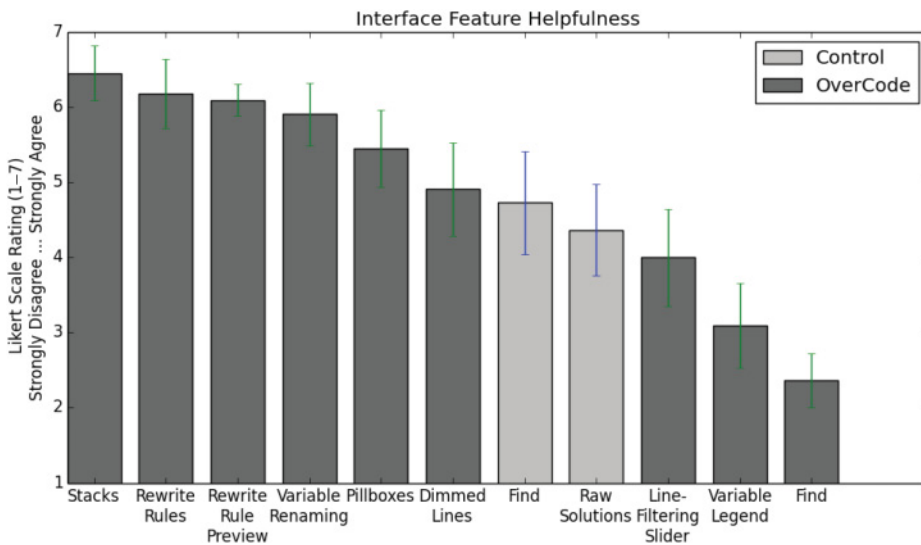
Fig. 22. Mean Likert scale ratings (with standard error) for the usefulness of features of OverCode and baseline. “Find” is the Web browser’s built-in find, which appears twice because users rated its usefulness for each condition.
