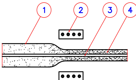
Figure 3: Schematics of stepped radial compression of rod-shaped or tubular parts.
