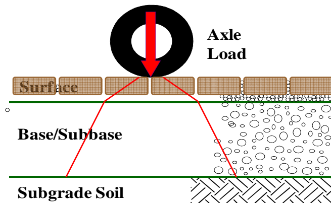
Figure 2. Distribution of traffic loads into underlying layers.
