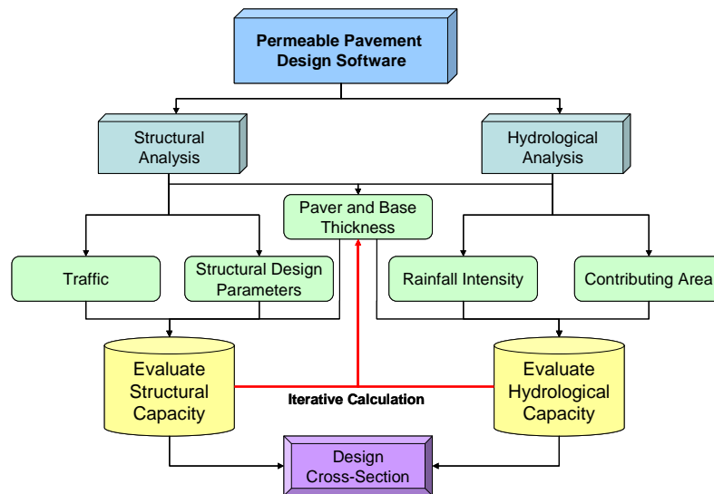
Figure 1. Flow chart of the permeable pavement design process.
