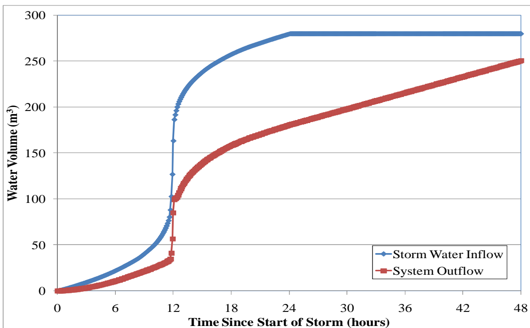
Figure 6. Comparison of PICP inflow vs. outflow.
