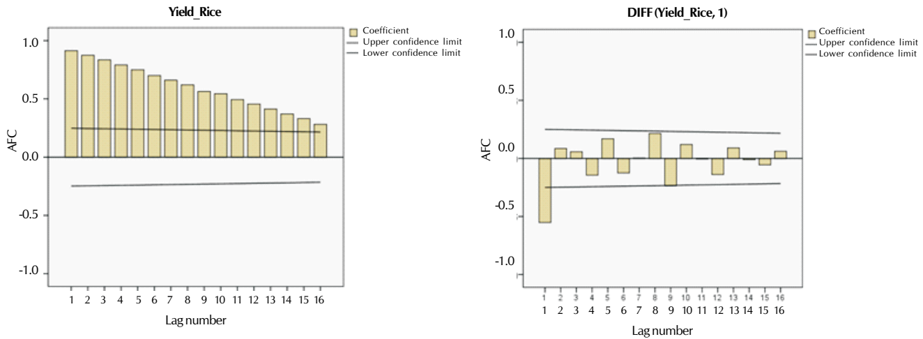
Figure 2: Autocorrelation Function of actual series (Yield_Rice) and differenced series (Yield_Rice_1)
