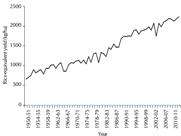
Figure 1: Yearly Trend of Rice Yield in India during 1950-51 to 2011-12
