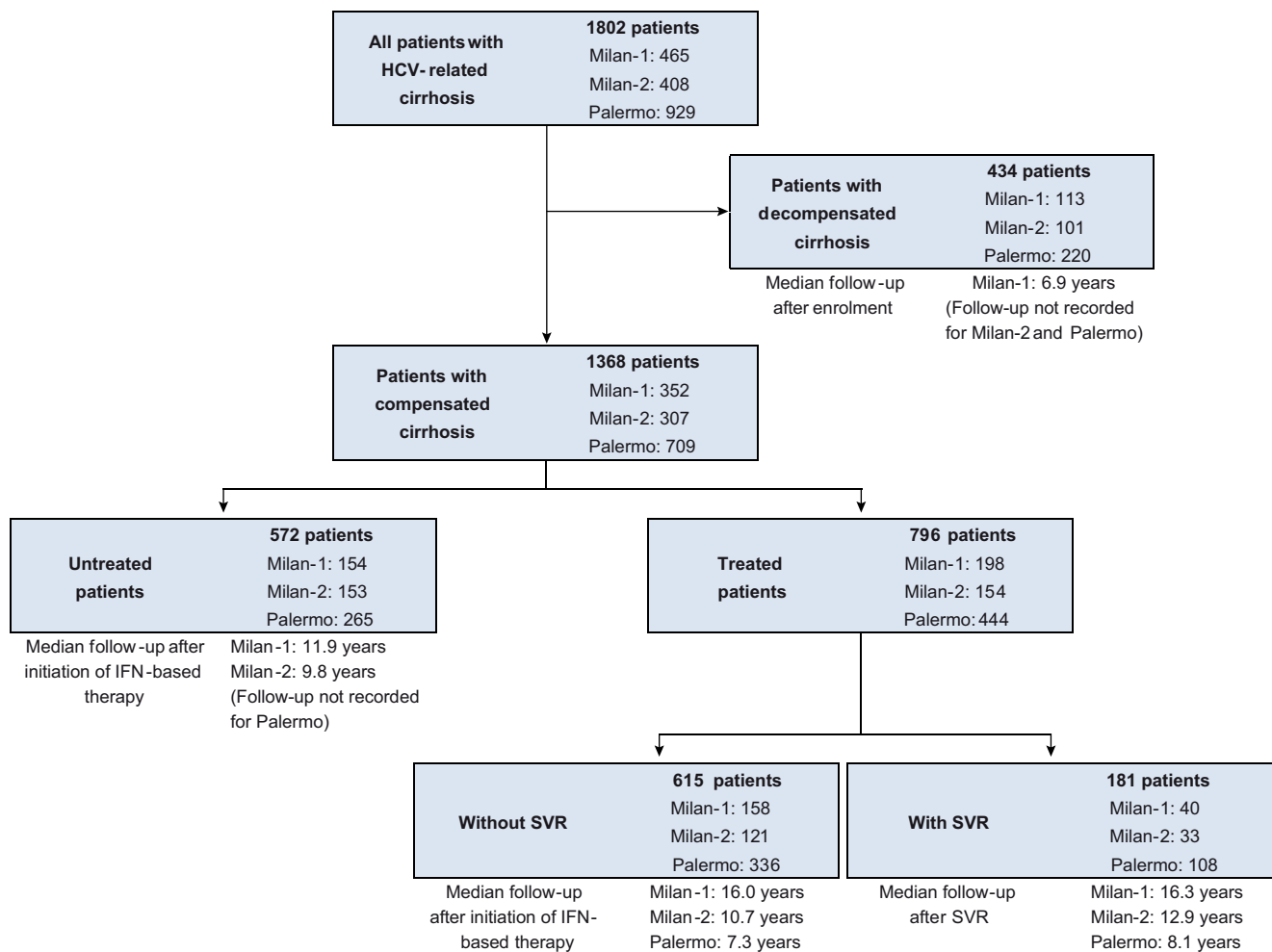
Fig. 1. Study flowchart.
