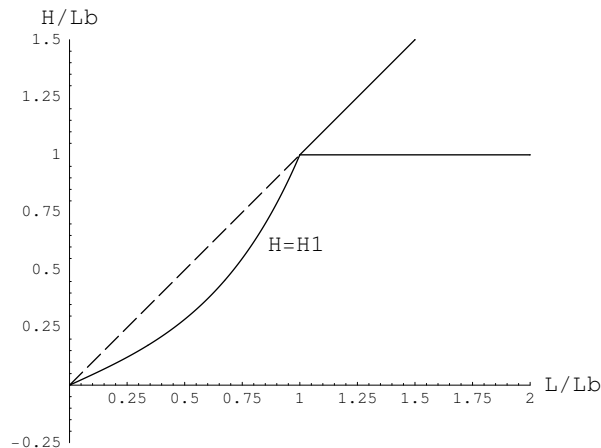
Figure 7: New version of fig.5 that includes the curve H_1(L/L_b) for L/L_b < 1 where highly deflected states disappear.
