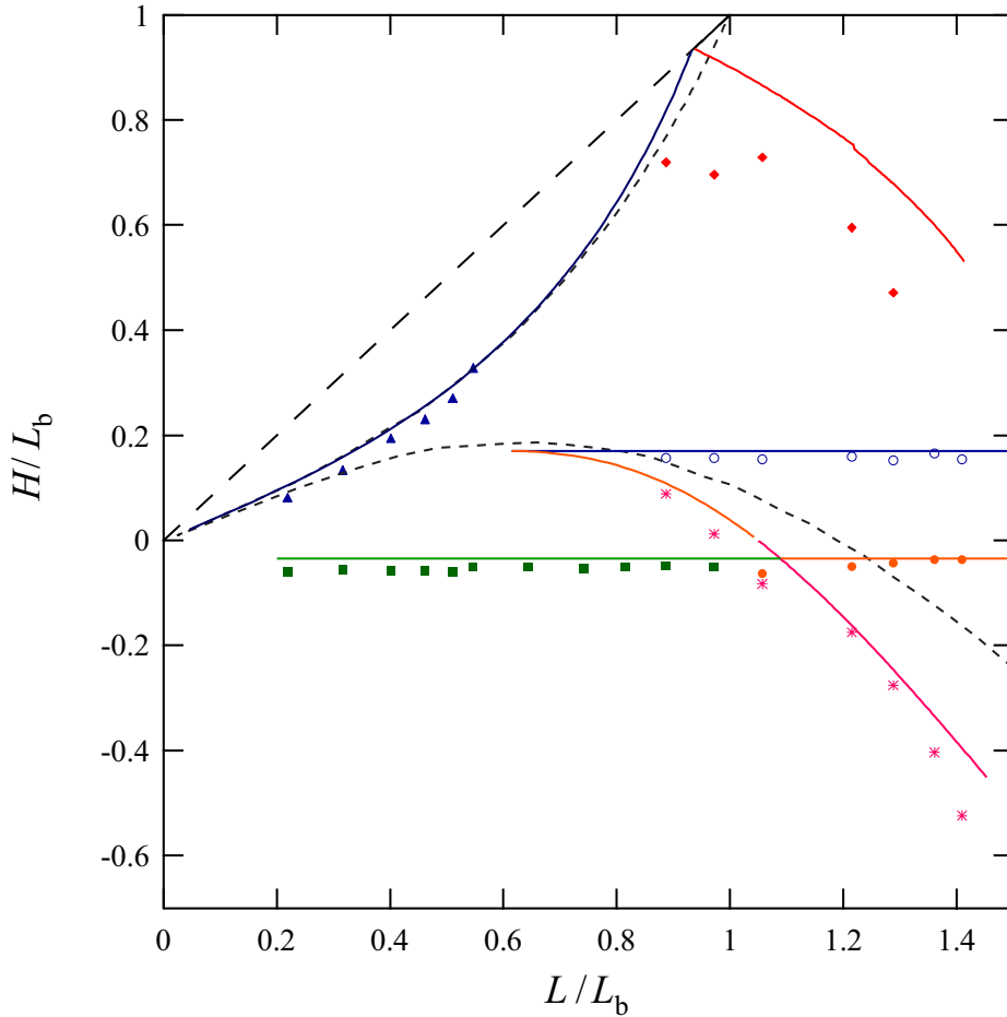
Figure 19: Experimental and numerical phase diagram for a fibre with a radius of 18 microns ( L_b = 9.8 cm). Experimental data is plotted as symbols, whereas numerical curves are in continuous line (with gravity) or dotted lines (without gravity).
