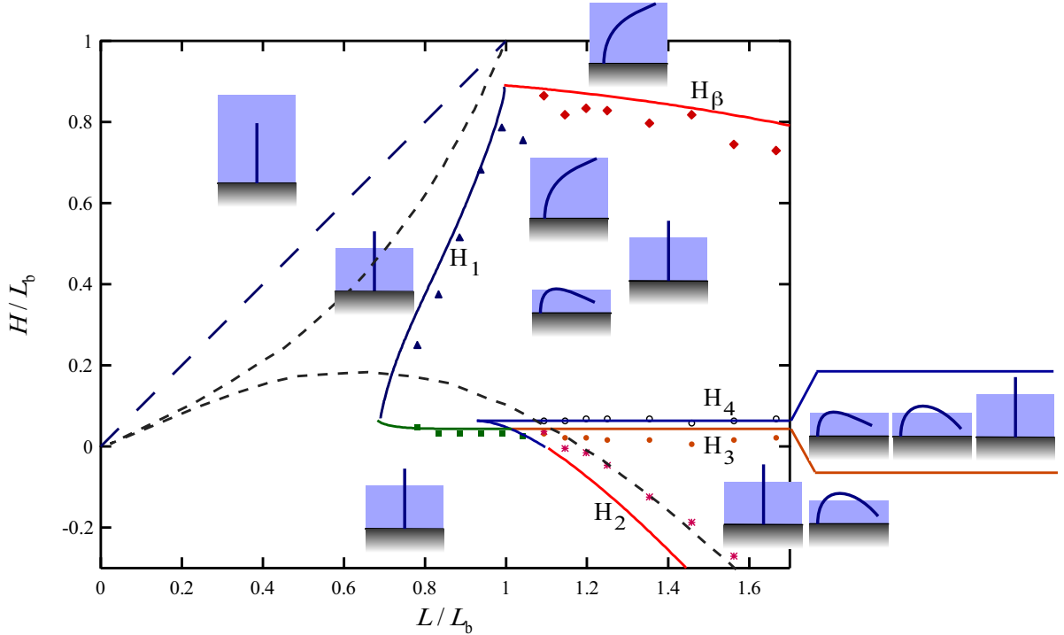
Figure 17: Experimental (symbols) and numerical (continuous lines) phase diagram for the elastic strip of thickness e = 25\mu\text{m} ( L_b = 1.9\text{ cm} ). In each region of the diagram the different stable configurations are sketched. The numerical computations include gravity and finite meniscus sizes, whereas dashed curves (corresponding to curves H_1 and H_2 ) obtained without gravity at zero capillary length ( L_c = 0 ) are drawn as guides to the eye.
