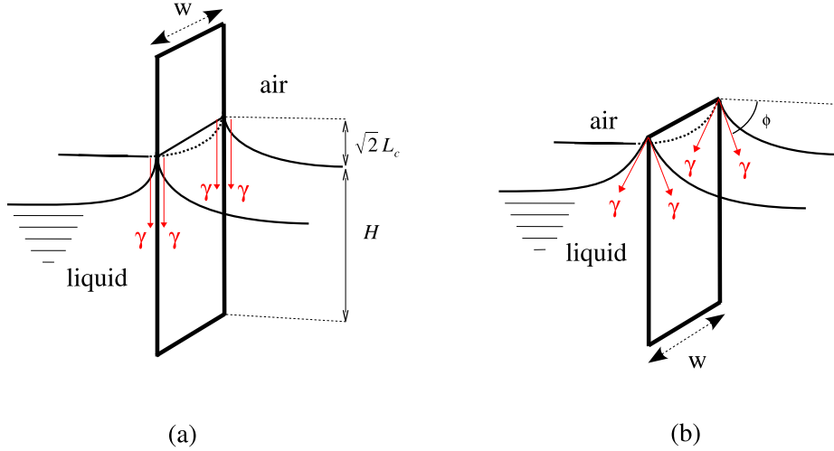
Figure 3: Elastic strip piercing (a) or only deflecting (b) a liquid surface. The (vertical) force provided by the liquid surface depends on the meniscus height.
