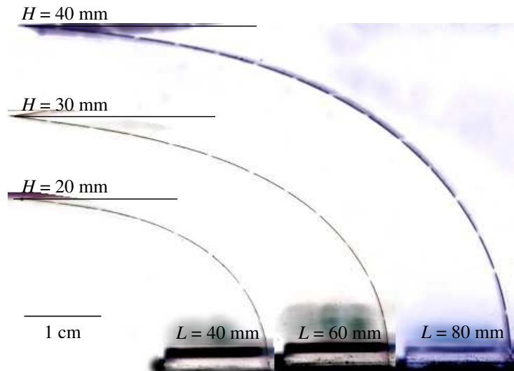
Figure 20: For the same ratio H/L , lightly deflected shapes are homothetic.
