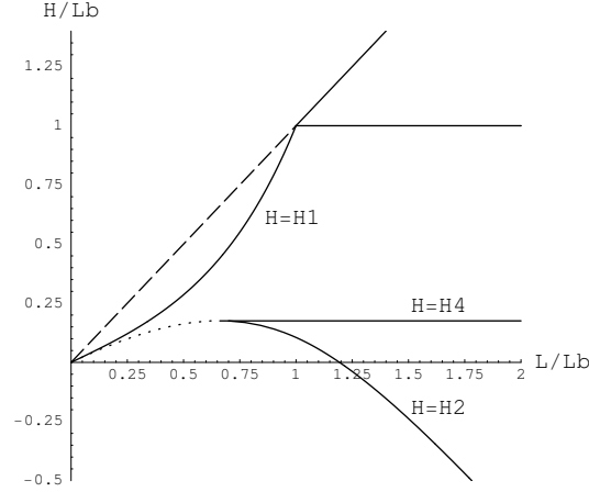
Figure 14: Extension of figure 9 where the curves corresponding to the two instabilities occurring for twice piercing states have been added (with L_b = 50L_c ). The curve H = H_2(L/L_b) , corresponding to configurations where the end of the beam emerges, connects with the curve introduced for the single piercing states (see fig.9). The dotted part of the H = H_2(L/L_b) curve is only plotted as a guide to the eye and does not correspond to any instability.
