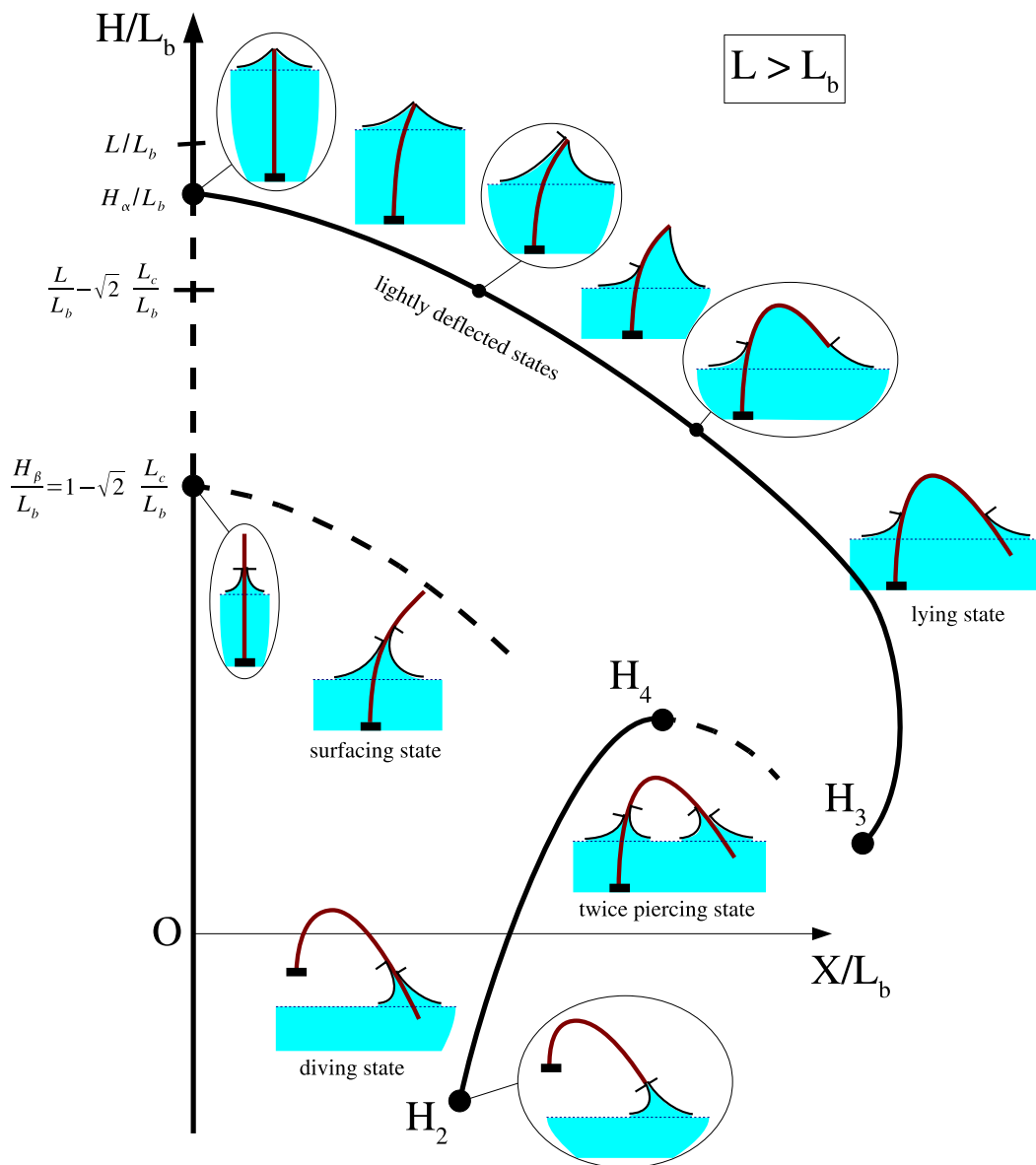
Figure 15: Typical bifurcation diagram for L > L_b showing the different equilibrium configurations. The parameters X and H correspond to the lateral position of the end of the beam and to the liquid height, respectively. Plain (resp. dotted) curves corresponds to stable (resp. unstable) states.
