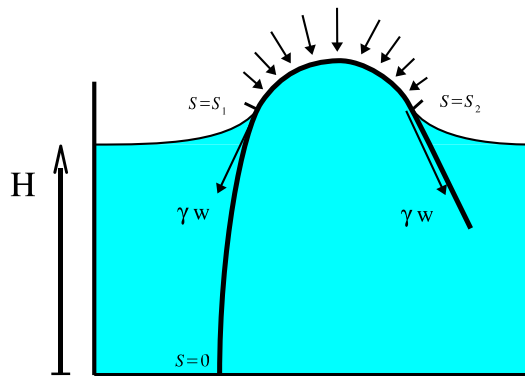
Figure 10: A lying configuration: at s = s_1 and s = s_2 , the interaction with the surface is modelled by discrete jumps in the inner force vector \mathbf{n}(s) . In the region s_1 < s < s_2 , the hydrostatic pressure yields a distributed force that is continuously changing \mathbf{n}(s) .
