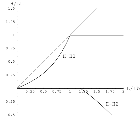
Figure 9: Extended version of fig.7 with the new curve H = H_2(L/L_b) where diving states lose stability as the end of the beam detaches from the interface.
