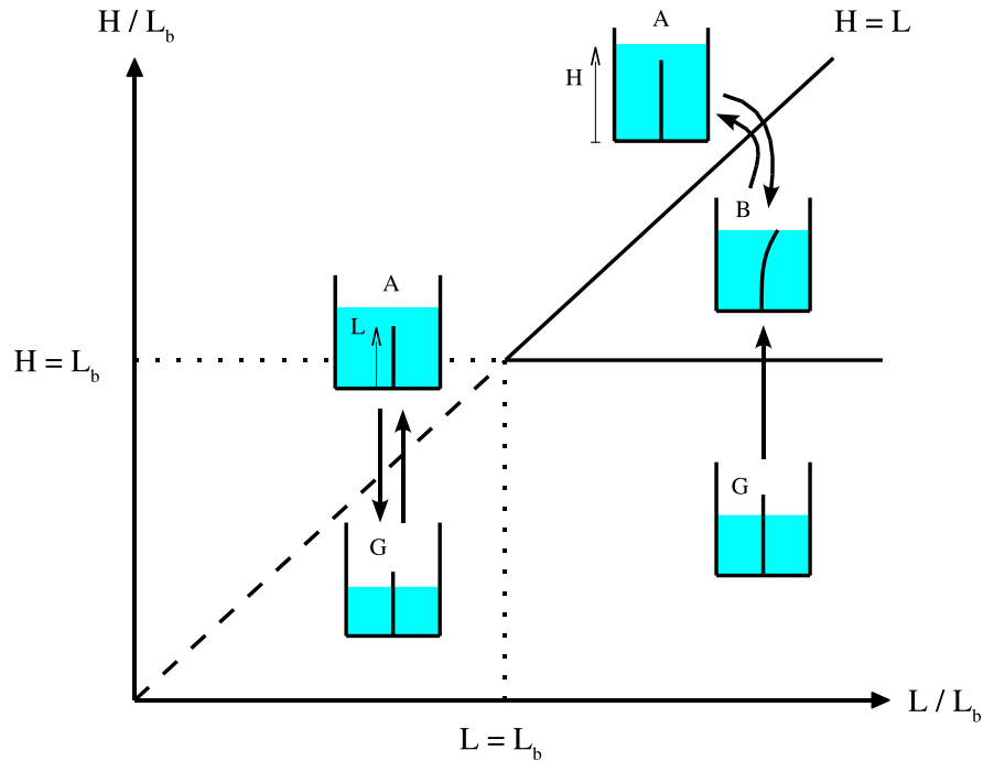
Figure 5: Parameter regimes for the buckling of a straight beam, of length L , by surface tension. Short beams ( L < L_b ) pierce the liquid interface whereas longer beams are deflected.
