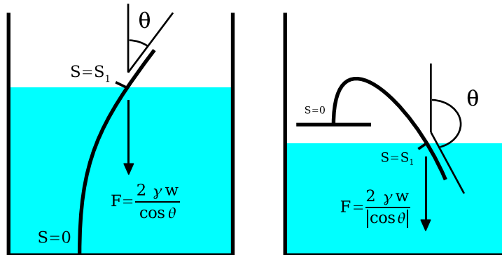
Figure 8: The two types of configuration of piercing states with L_c = 0 . (Left) Surfacing state. These states are always unstable. (Right) Diving state. These states exist when L/L_b > 1.2 and H_2 < H < 0 .
