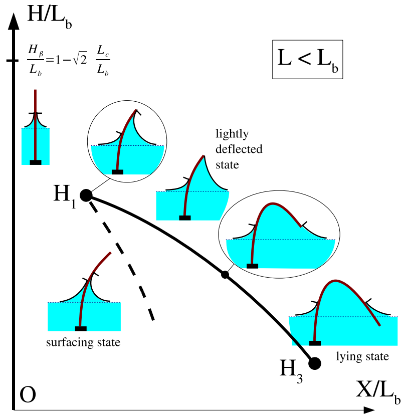
Figure 16: Typical bifurcation diagram for L < L_b showing the different equilibrium configurations. The parameters X and H correspond to the lateral position of the end of the beam and to the liquid height, respectively. Plain (resp. dotted) curves corresponds to stable (resp. unstable) states.
