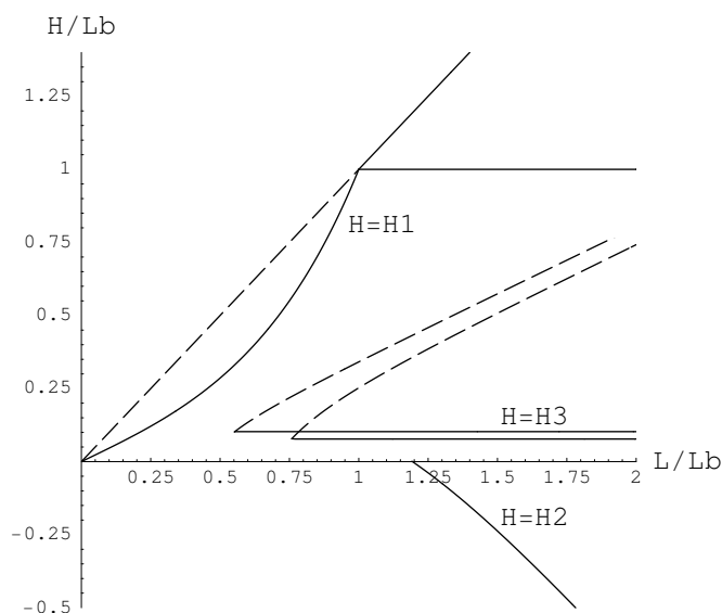
Figure 11: Extended version of figure 9 where curves corresponding to the lying state instabilities have been added. The horizontal lines ( H = H_3 ) correspond to configurations where the liquid arch detaches from the beam (lower line for L_b = 20L_c , upper one for L_b = 50L_c ). The oblique nearly straight curve corresponds to configurations where the end of the beam enters/exits the liquid (lower curve for L_b = 20L_c , upper one for L_b = 50L_c ). The other curves ( H_1, H_2 , etc) are computed in the zero L_c approximation.
