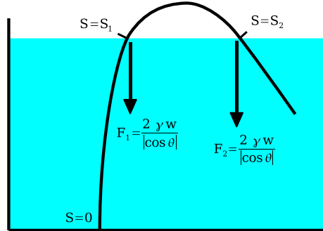
Figure 13: Twice piercing state. In the present zero capillary length approximation, left and right menisci at both crossing points ( s_1 and s_2 ) are replaced by point forces.
