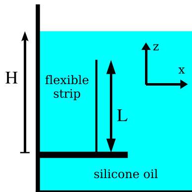
Figure 1: Experimental setup : an elastic strip or a fibre is clamped at its base on a horizontal rigid support. We lower/raise the support along a pole so that the strip gradually emerges from the bath of silicone oil.
