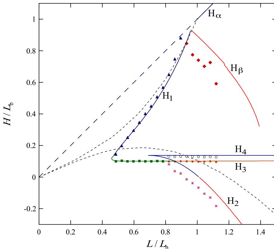
Figure 18: Experimental and numerical phase diagram for the elastic strip of thickness e = 50\mu\text{m} ( L_b = 6.0\text{ cm} ). Dotted curves, corresponding to curves H_1 and H_2 at zero capillary length ( L_c = 0 ) are drawn as guides to the eye.
