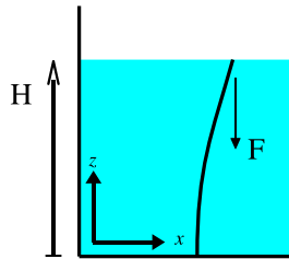
Figure 6: Lightly deflected state at null capillary length ( L_c = 0 ): the meniscus size is neglected, and the force F is an unknown of the boundary value problem.
