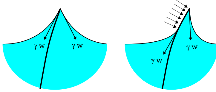
Figure 12: The two different types of configurations of lightly deflected states at non-zero L_c . Left: the two menisci joining the apex of the beam to the asymptotical bath height H are vertically symmetric. Right: the beam has a semi-submerged part.
