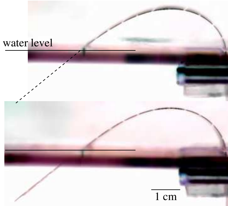
Figure 21: Free end configurations may always be lengthened without change. These two configurations with the same bath height have different lengths but an identical emerged part.
