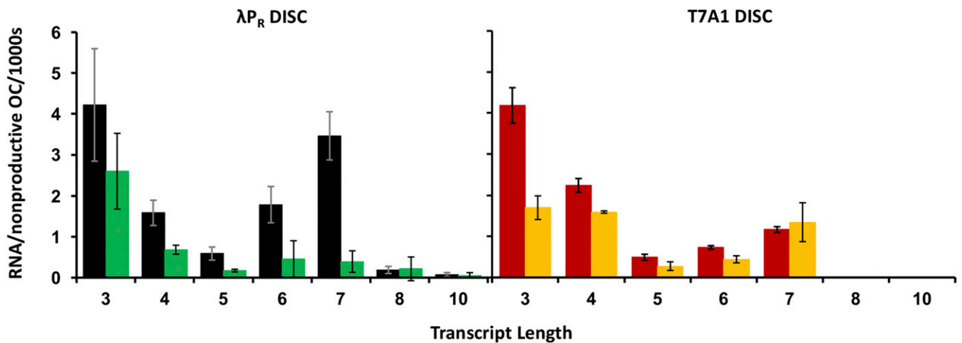
Fig. 5. Rates of synthesis of short RNAs per nonproductive (i.e., abortively initiating) OC in the slower phase of transcription initiation. Bar graphs summarize steady-state synthesis rates for all short RNAs synthesized in the linear (slow, abortive) phase from promoters with \lambda P_R (Left) and T7A1 (Right) discriminators (DISC). Rates are the averages obtained from best-fit slopes of the linear (steady-state) regions of two to four kinetics experiments \pm standard error (see example in SI Appendix, Fig. S6 and Table S6 ) and are expressed as the number of RNAs synthesized per nonproductive promoter OC per 1,000 s. Color-coding is the same as in Fig. 4.
