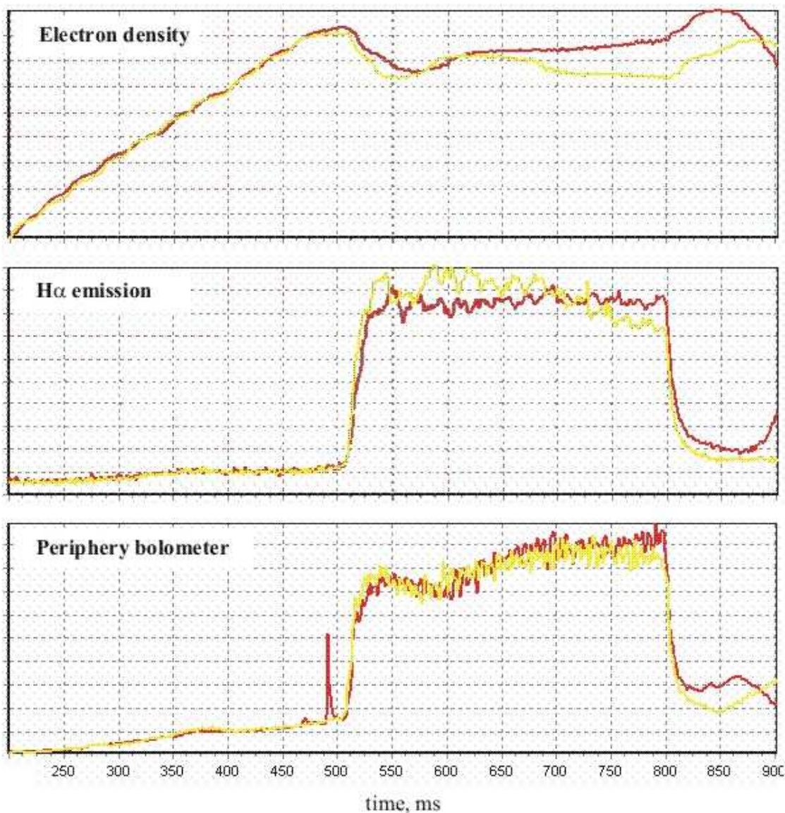
Fig. 1. Evolution of main plasma parameters in the reference shots before (#42312 red curve) and after (#42319 yellow curve) series with Li injection. All data are in arbitrary units.
