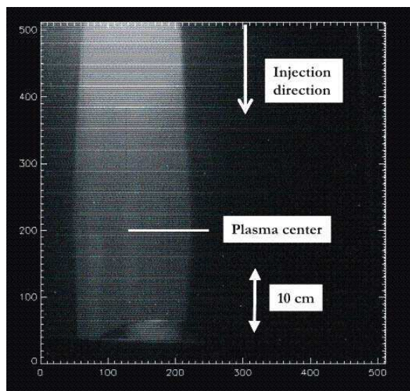
Fig. 3. He supersonic jet penetration in T-10 plasma.
