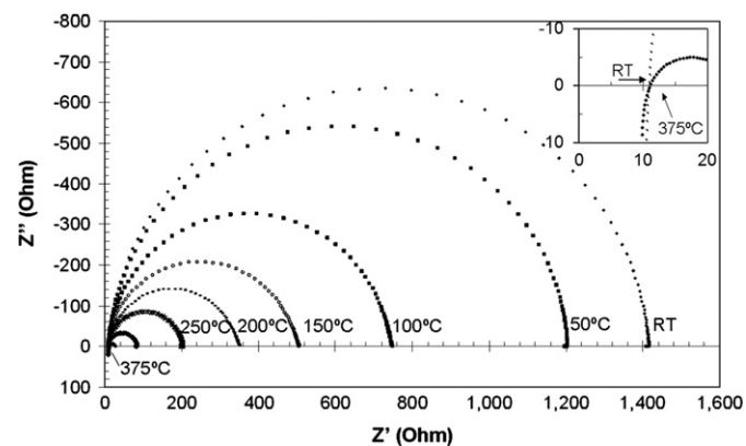
Fig. 3. Impedance plot for Ti_nO_{2n-1} (1 MHz to 0.1 Hz, RT to 375^\circ C ). The inset shows the non-zero intercept on the Z' axes, from which the resistance ( R_B ) of the grain bulk can be obtained. The only observable arc is attributed to the grain boundaries ( R_{GB} ) response.
