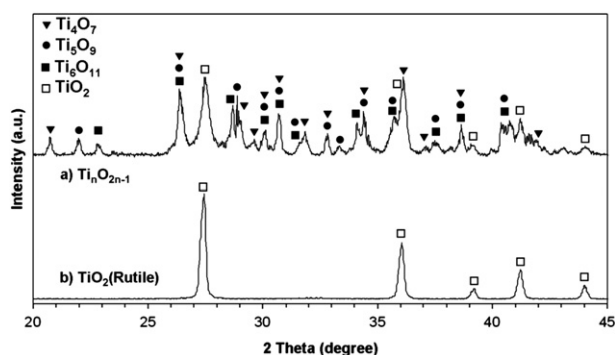
Fig. 2. XRD spectra of Ti_nO_{2n-1} obtained from carbothermal reduction (a) and TiO_2 before the reduction step (b).
