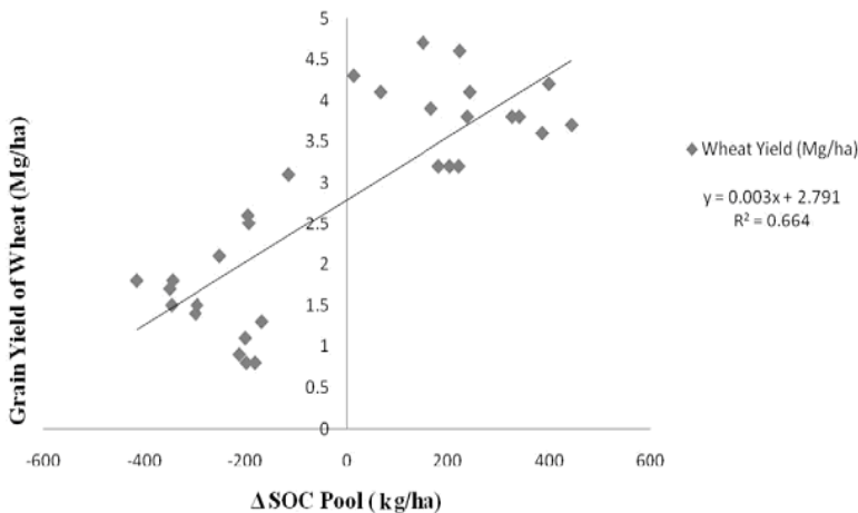
Figure 7. Effect of changes in soil organic carbon (ΔSOC) pool in the root zone on grain yield of wheat in Australia (redrawn and recalculated from Farquharson et al., 2003).
