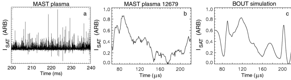
Figure 1: Isat signals
