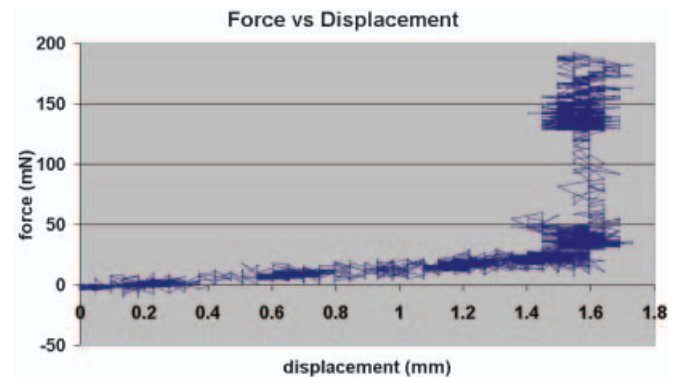
Figure 6 Relation between experimentally obtained force and displacement recorded during vessel occlusion. An abrupt jump in the force applied occurs when the vessel is fully occluded. The jagged lines were caused due to pulsation and tissue relaxation of the aorta, and the noise of the system.
