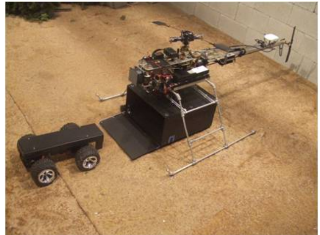
Figure 1. A belly-mounted docking station permits the robotic helicopter to aerially transport an unmanned ground vehicle
