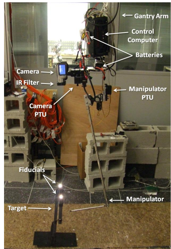
Figure 4. Cargo Pickup Mechanism
