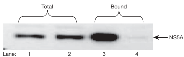
Figure 2 | The active inhibitor 1 binds to genotype 1b HCV NS5A whereas the inactive stereoisomer 2 does not. Genotype 1b replicon cells were exposed to either 1 or 2 for approximately 18 h before the cells were lysed. A portion of the supernatant was set aside to serve as input control for immunoblot analysis (lanes 1 and 2) while the remainder was mixed with streptavidin-agarose beads and incubated for several hours. Bound proteins were detected by immunoblotting with primary antibodies directed to HCV NS5A. Lanes 1 and 3 depict the results of experiments with the active inhibitor compound 1 whereas lanes 2 and 4 depict the results with the inactive stereoisomer 2.
