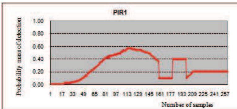
Fig. 2.1. Output pattern of PIR1 located in zone 0
