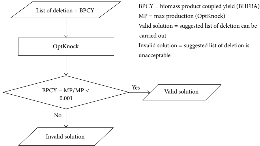
FIGURE 5: The flow of OptKnock validation.
